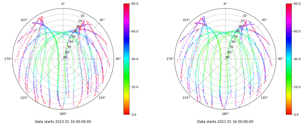
Skyplot for station LALA. Parameter M1C Data file LALA00ESP_R_2023016.xtr Skyplot for station LALA. Parameter M2C Data file LALA00ESP_R_2023016.xtr
