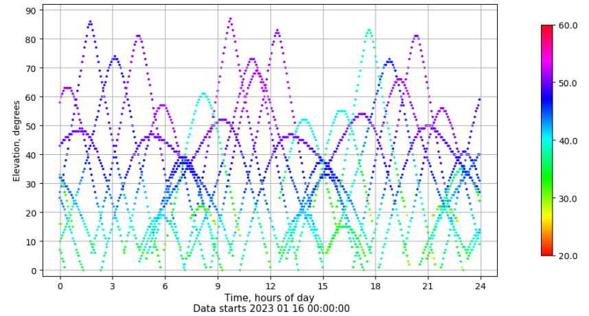
Time-elevation plot for station LALA. Signal to Noise S1C Data file LALA00ESP_R_2023016.xtr
