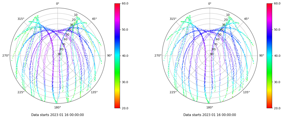
Skyplot for station LALA. Signal to Noise S1C Data file LALA00ESP_R_2023016.xtr Skyplot for station LALA. Signal to Noise S2C Data file LALA00ESP_R_2023016.xtr
