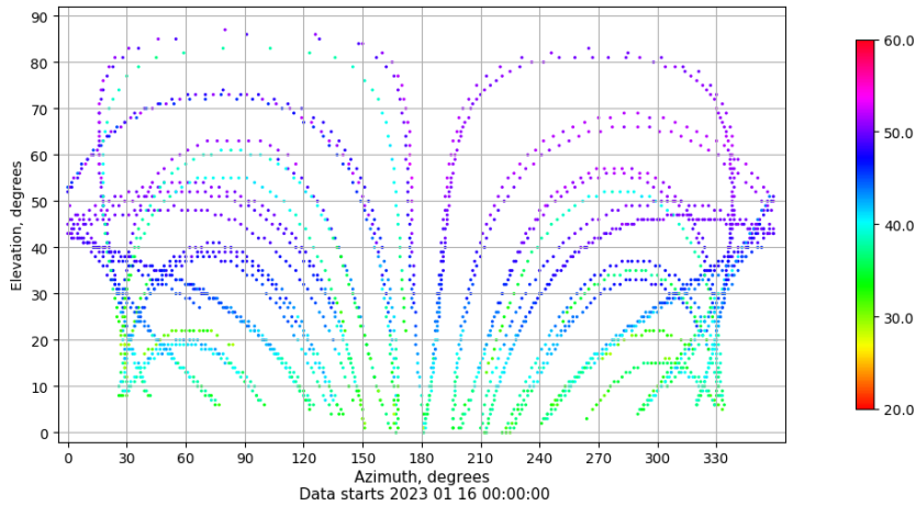
Azimuth-elevation plot for station LALA. Signal to Noise S1C Data file LALA00ESP_R_2023016.xtr
