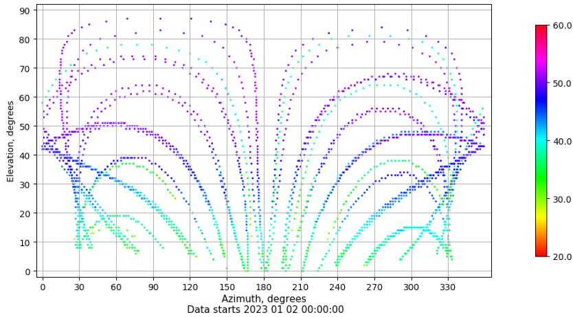
Azimuth-elevation plot for station LALA. Signal to Noise S1C Data file LALA00ESP_R_2023002.xtr
