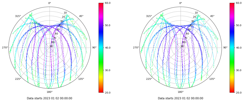
Skyplot for station LALA. Signal to Noise S1C Data file LALA00ESP_R_2023002.xtr Skyplot for station LALA. Signal to Noise S2C Data file LALA00ESP_R_2023002.xtr
