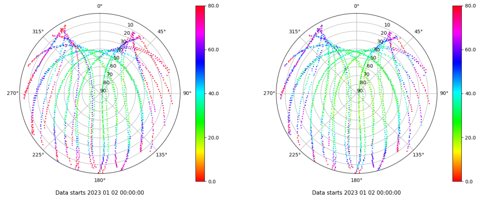
Skyplot for station LALA. Parameter M1C Data file LALA00ESP_R_2023002.xtr Skyplot for station LALA. Parameter M2C Data file LALA00ESP_R_2023002.xtr
