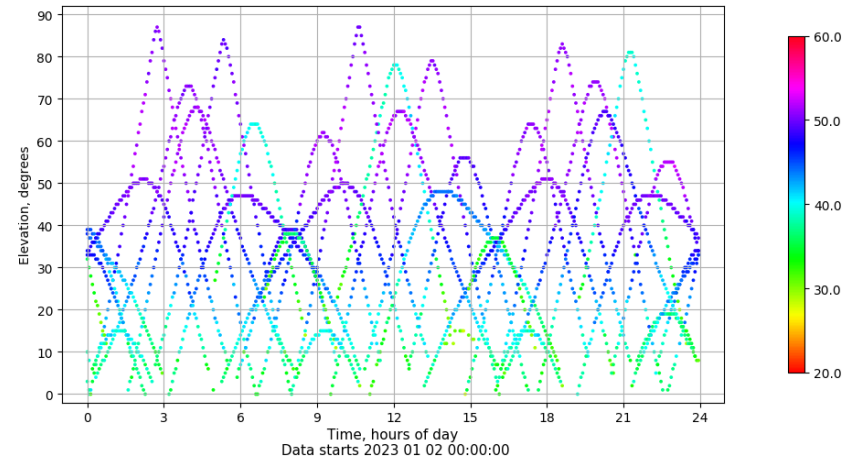
Time-elevation plot for station LALA. Signal to Noise S1C Data file LALA00ESP_R_2023002.xtr
