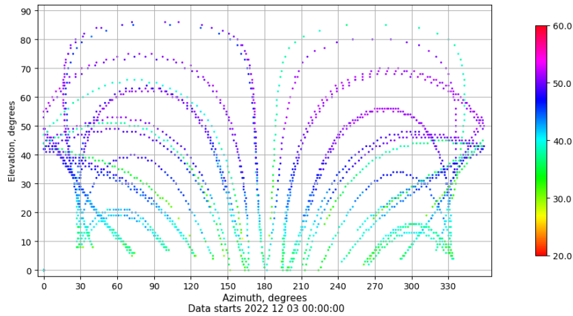
Azimuth-elevation plot for station LALA. Signal to Noise S1C Data file LALA00ESP_R_2022337.xtr
