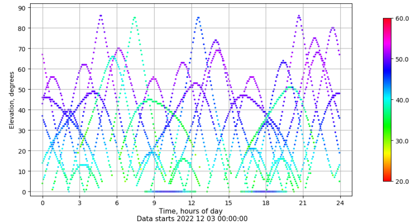
Time-elevation plot for station LALA. Signal to Noise S1C Data file LALA00ESP_R_2022337.xtr
