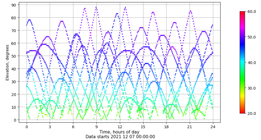
Time-elevation plot for station LALA. Signal to Noise S1C Data file LALA00ESP_R_2021341.xtr
