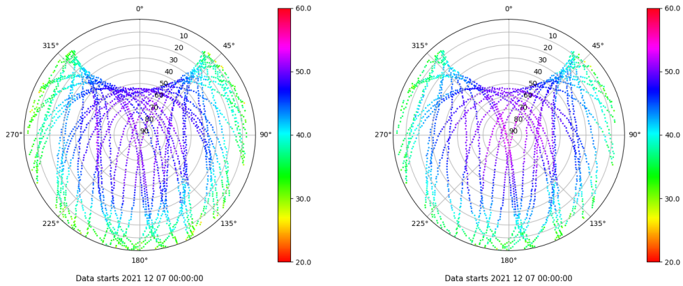
Skyplot for station LALA. Signal to Noise S1C Data file LALA00ESP_R_2021341.xtr Skyplot for station LALA. Signal to Noise S2X Data file LALA00ESP_R_2021341.xtr
