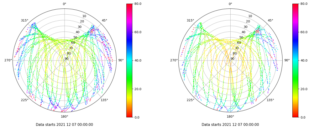
Skyplot for station LALA. Parameter M1C Data file LALA00ESP_R_2021341.xtr Skyplot for station LALA. Parameter M2X Data file LALA00ESP_R_2021341.xtr
