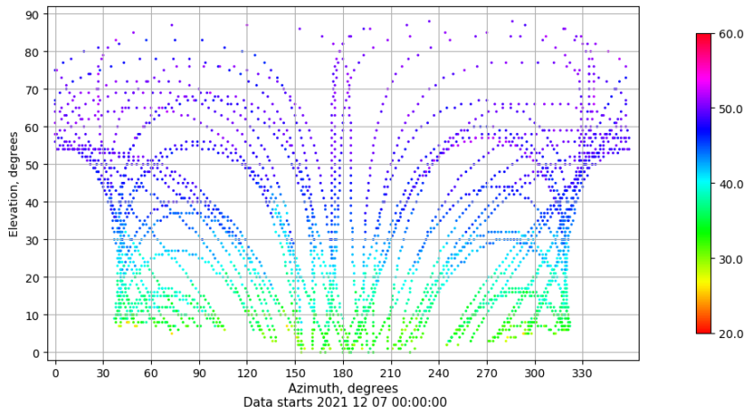
Azimuth-elevation plot for station LALA. Signal to Noise S1C Data file LALA00ESP_R_2021341.xtr
