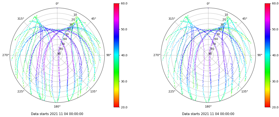
Skyplot for station LALA. Signal to Noise S1C Data file LALA00ESP_R_2021308.xtr Skyplot for station LALA. Signal to Noise S2C Data file LALA00ESP_R_2021308.xtr
