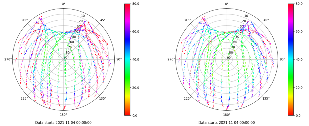
Skyplot for station LALA. Parameter M1C Data file LALA00ESP_R_2021308.xtr Skyplot for station LALA. Parameter M2C Data file LALA00ESP_R_2021308.xtr
