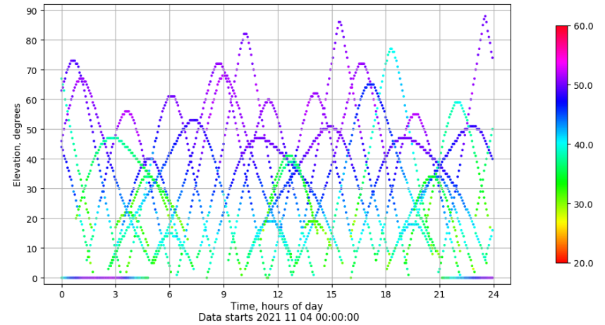
Time-elevation plot for station LALA. Signal to Noise S1C Data file LALA00ESP_R_2021308.xtr
