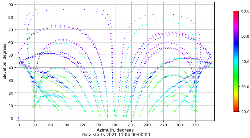
Azimuth-elevation plot for station LALA. Signal to Noise S1C Data file LALA00ESP_R_2021308.xtr
