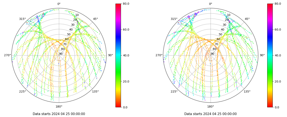
Skyplot for station JACA. Parameter M1C Data file JACA00ESP_R_2024116.xtr Skyplot for station JACA. Parameter M2P Data file JACA00ESP_R_2024116.xtr
