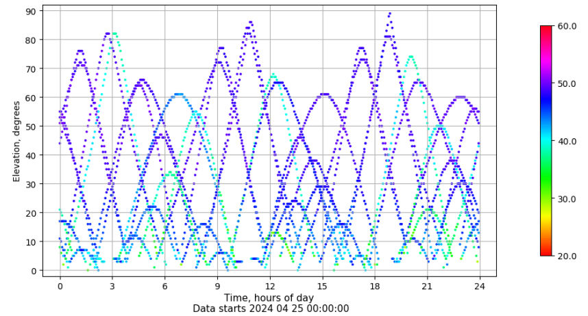
Time-elevation plot for station JACA. Signal to Noise S1C Data file JACA00ESP_R_2024116.xtr
