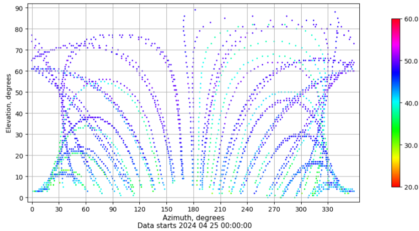
Azimuth-elevation plot for station JACA. Signal to Noise S1C Data file JACA00ESP_R_2024116.xtr
