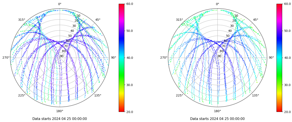
Skyplot for station JACA. Signal to Noise S1C Data file JACA00ESP_R_2024116.xtr Skyplot for station JACA. Signal to Noise S2P Data file JACA00ESP_R_2024116.xtr
