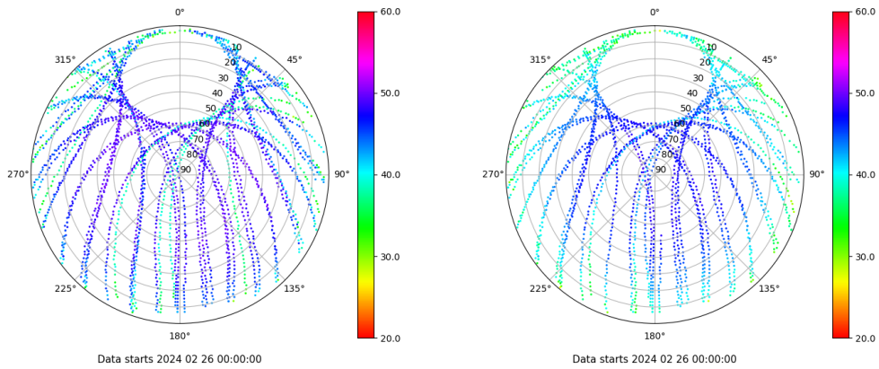
Skyplot for station JACA. Signal to Noise S1C Data file JACA00ESP_R_2024057.xtr Skyplot for station JACA. Signal to Noise S2P Data file JACA00ESP_R_2024057.xtr
