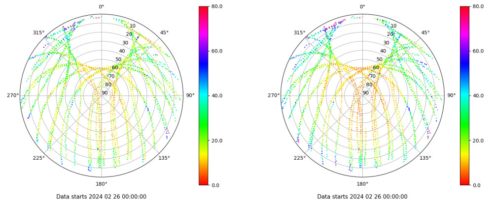
Skyplot for station JACA. Parameter M1C Data file JACA00ESP_R_2024057.xtr Skyplot for station JACA. Parameter M2P Data file JACA00ESP_R_2024057.xtr
