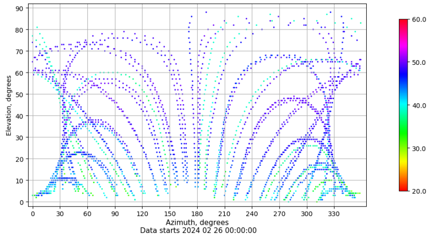
Azimuth-elevation plot for station JACA. Signal to Noise S1C Data file JACA00ESP_R_2024057.xtr
