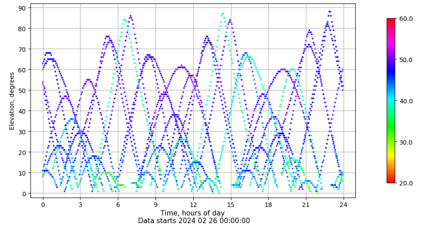
Time-elevation plot for station JACA. Signal to Noise S1C Data file JACA00ESP_R_2024057.xtr
