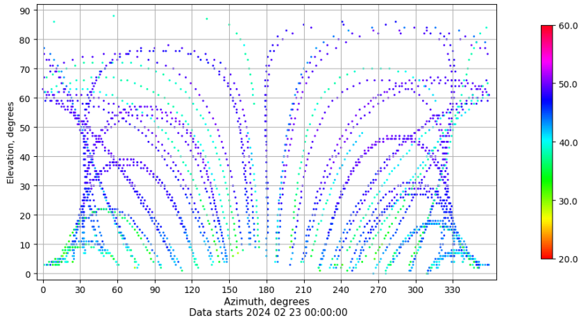
Azimuth-elevation plot for station JACA. Signal to Noise S1C Data file JACA00ESP_R_2024054.xtr
