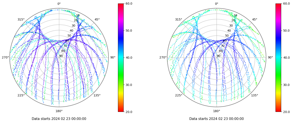
Skyplot for station JACA. Signal to Noise S1C Data file JACA00ESP_R_2024054.xtr Skyplot for station JACA. Signal to Noise S2P Data file JACA00ESP_R_2024054.xtr
