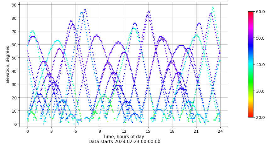
Time-elevation plot for station JACA. Signal to Noise S1C Data file JACA00ESP_R_2024054.xtr
