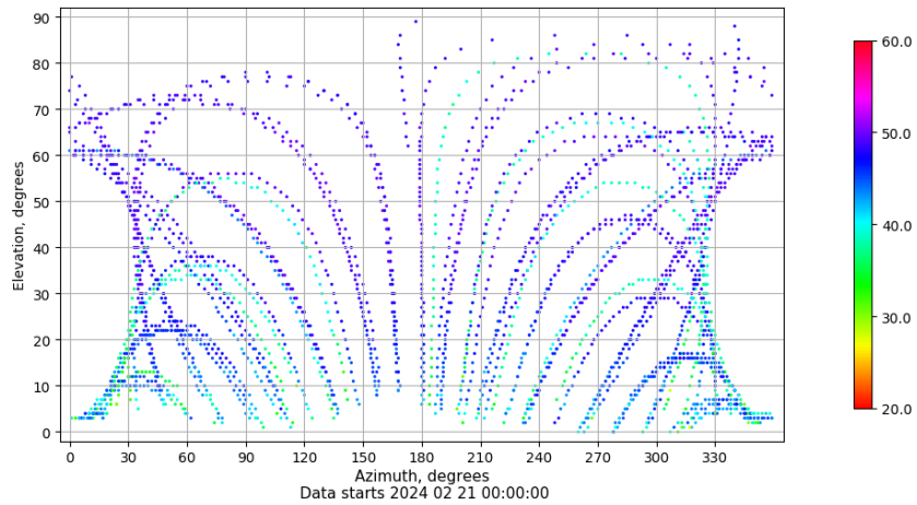
Azimuth-elevation plot for station JACA. Signal to Noise S1C Data file JACA00ESP_R_2024052.xtr
