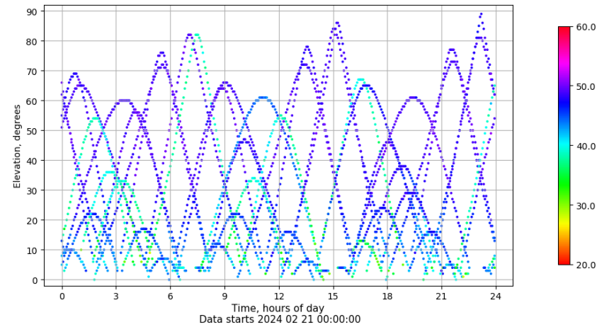
Time-elevation plot for station JACA. Signal to Noise S1C Data file JACA00ESP_R_2024052.xtr
