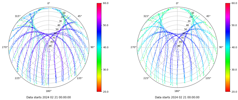
Skyplot for station JACA. Signal to Noise S1C Data file JACA00ESP_R_2024052.xtr Skyplot for station JACA. Signal to Noise S2P Data file JACA00ESP_R_2024052.xtr
