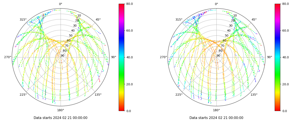
Skyplot for station JACA. Parameter M1C Data file JACA00ESP_R_2024052.xtr Skyplot for station JACA. Parameter M2P Data file JACA00ESP_R_2024052.xtr
