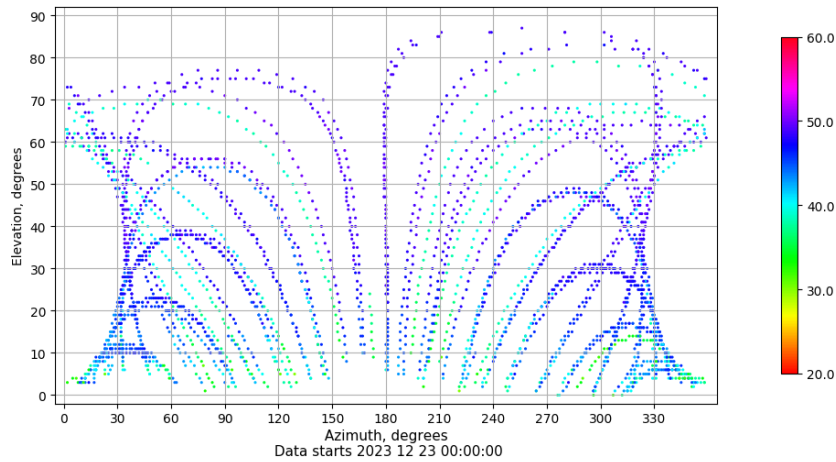
Azimuth-elevation plot for station JACA. Signal to Noise S1C Data file JACA00ESP_R_2023357.xtr
