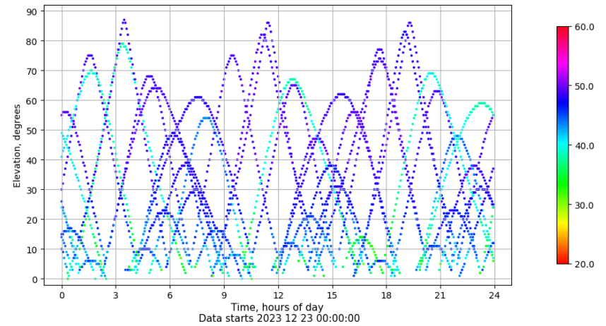
Time-elevation plot for station JACA. Signal to Noise S1C Data file JACA00ESP_R_2023357.xtr
