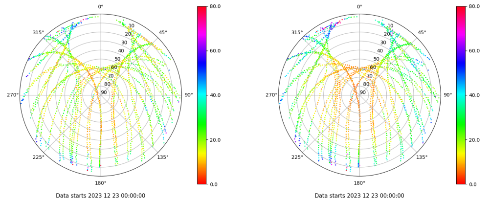
Skyplot for station JACA. Parameter M1C Data file JACA00ESP_R_2023357.xtr Skyplot for station JACA. Parameter M2P Data file JACA00ESP_R_2023357.xtr
