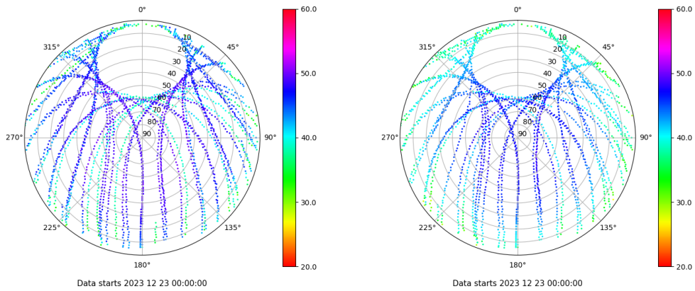
Skyplot for station JACA. Signal to Noise S1C Data file JACA00ESP_R_2023357.xtr Skyplot for station JACA. Signal to Noise S2P Data file JACA00ESP_R_2023357.xtr
