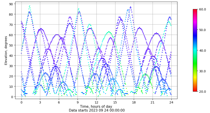
Time-elevation plot for station JACA. Signal to Noise S1C Data file JACA00ESP_R_2023267.xtr
