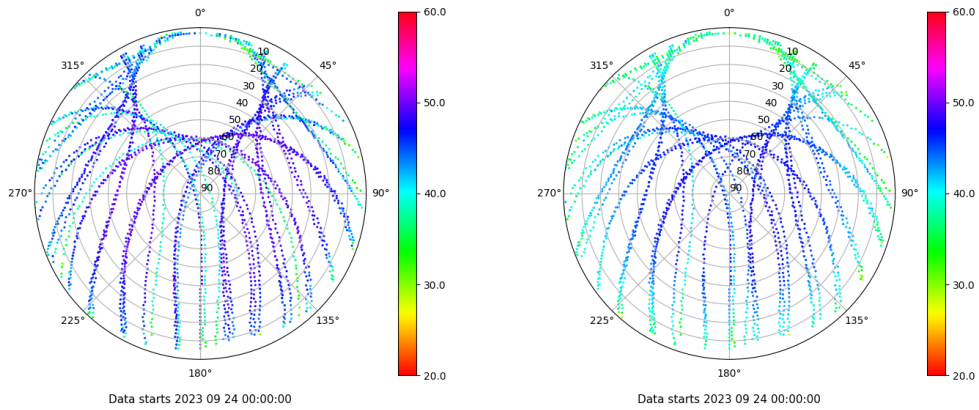
Skyplot for station JACA. Signal to Noise S1C Data file JACA00ESP_R_2023267.xtr Skyplot for station JACA. Signal to Noise S2P Data file JACA00ESP_R_2023267.xtr
