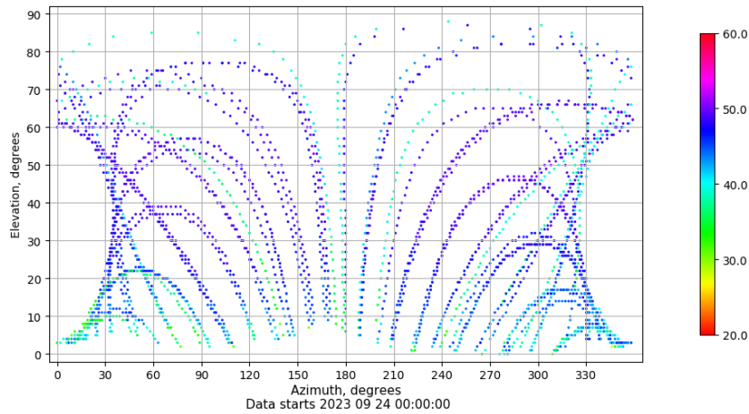
Azimuth-elevation plot for station JACA. Signal to Noise S1C Data file JACA00ESP_R_2023267.xtr
