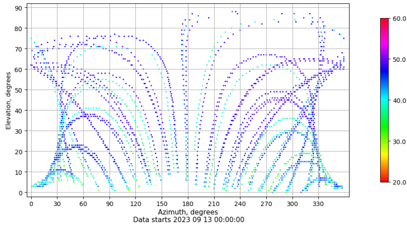
Azimuth-elevation plot for station JACA. Signal to Noise S1C Data file JACA00ESP_R_2023256.xtr
