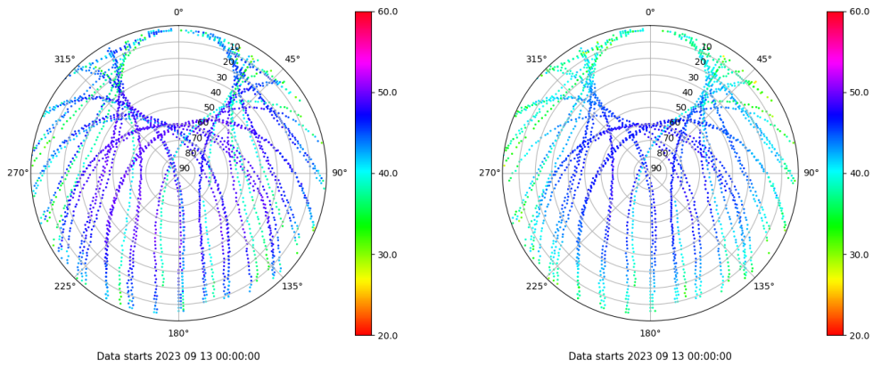
Skyplot for station JACA. Signal to Noise S1C Data file JACA00ESP_R_2023256.xtr Skyplot for station JACA. Signal to Noise S2P Data file JACA00ESP_R_2023256.xtr
