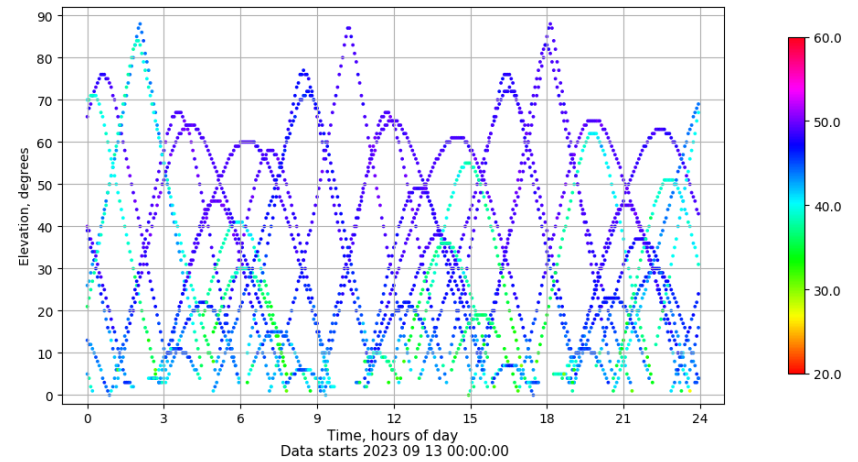
Time-elevation plot for station JACA. Signal to Noise S1C Data file JACA00ESP_R_2023256.xtr
