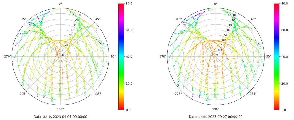
Skyplot for station JACA. Parameter M1C Data file JACA00ESP_R_2023250.xtr Skyplot for station JACA. Parameter M2P Data file JACA00ESP_R_2023250.xtr
