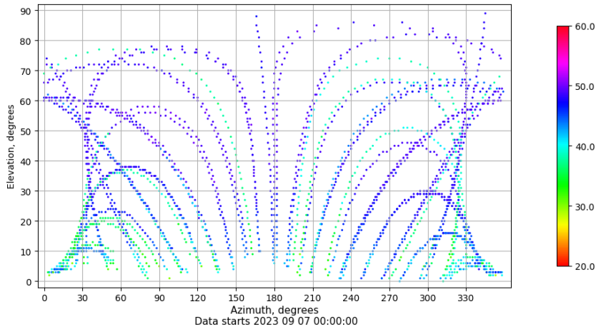
Azimuth-elevation plot for station JACA. Signal to Noise S1C Data file JACA00ESP_R_2023250.xtr
