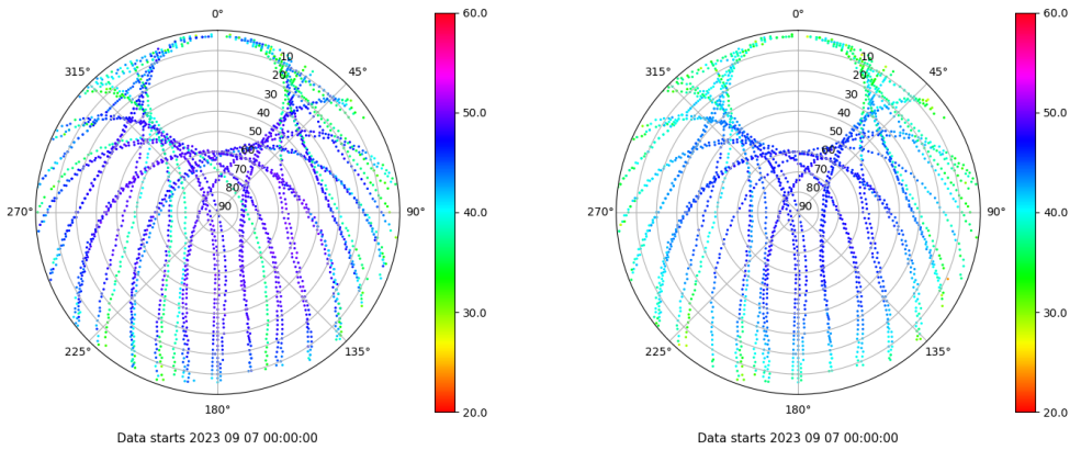
Skyplot for station JACA. Signal to Noise S1C Data file JACA00ESP_R_2023250.xtr Skyplot for station JACA. Signal to Noise S2P Data file JACA00ESP_R_2023250.xtr
