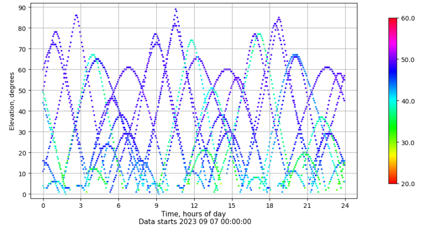
Time-elevation plot for station JACA. Signal to Noise S1C Data file JACA00ESP_R_2023250.xtr
