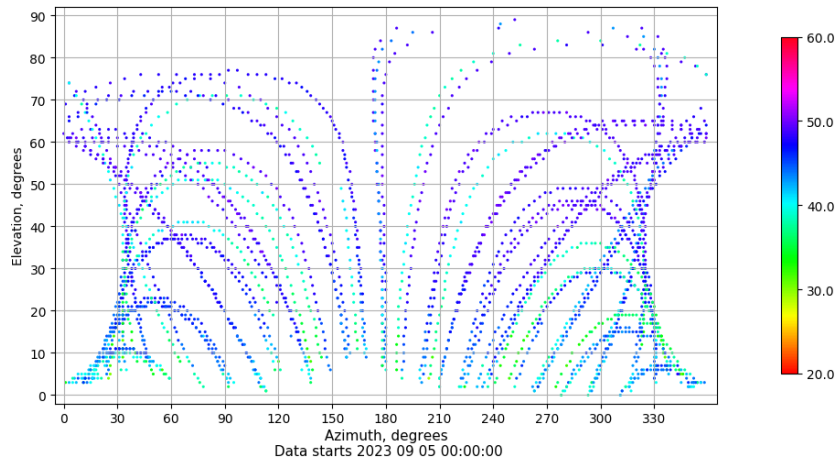
Azimuth-elevation plot for station JACA. Signal to Noise S1C Data file JACA00ESP_R_2023248.xtr
