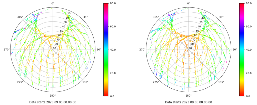
Skyplot for station JACA. Parameter M1C Data file JACA00ESP_R_2023248.xtr Skyplot for station JACA. Parameter M2P Data file JACA00ESP_R_2023248.xtr
