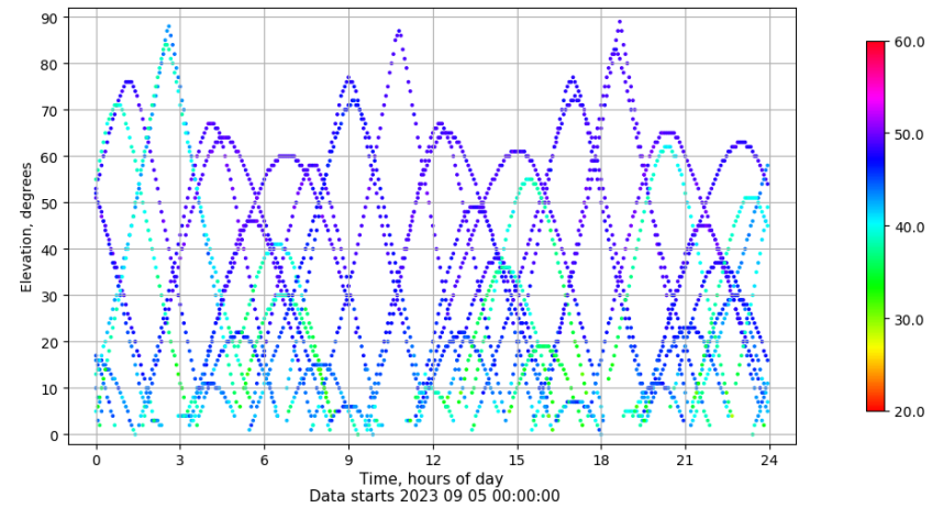
Time-elevation plot for station JACA. Signal to Noise S1C Data file JACA00ESP_R_2023248.xtr
