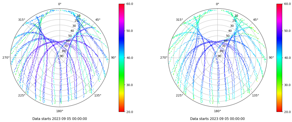
Skyplot for station JACA. Signal to Noise S1C Data file JACA00ESP_R_2023248.xtr Skyplot for station JACA. Signal to Noise S2P Data file JACA00ESP_R_2023248.xtr
