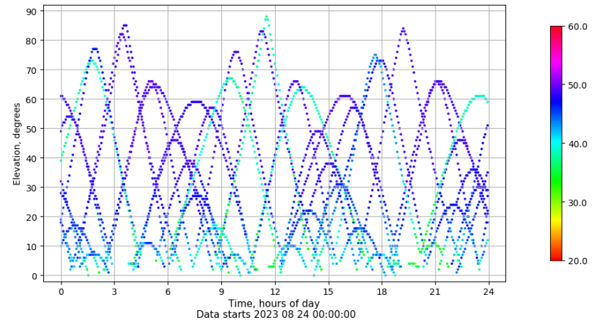
Time-elevation plot for station JACA. Signal to Noise S1C Data file JACA00ESP_R_2023236.xtr
