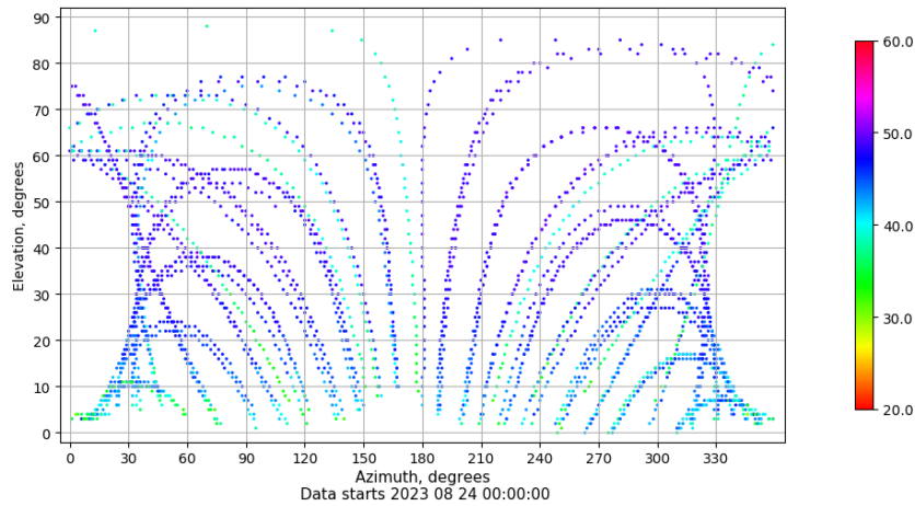
Azimuth-elevation plot for station JACA. Signal to Noise S1C Data file JACA00ESP_R_2023236.xtr
