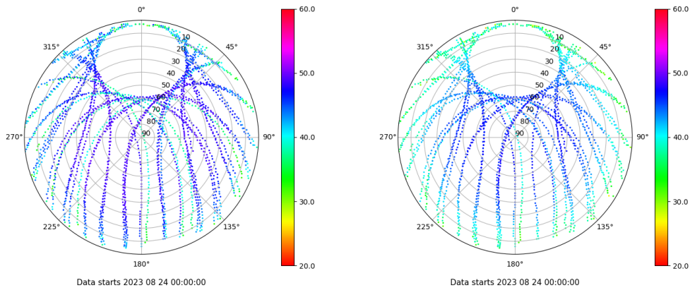
Skyplot for station JACA. Signal to Noise S1C Data file JACA00ESP_R_2023236.xtr Skyplot for station JACA. Signal to Noise S2P Data file JACA00ESP_R_2023236.xtr
