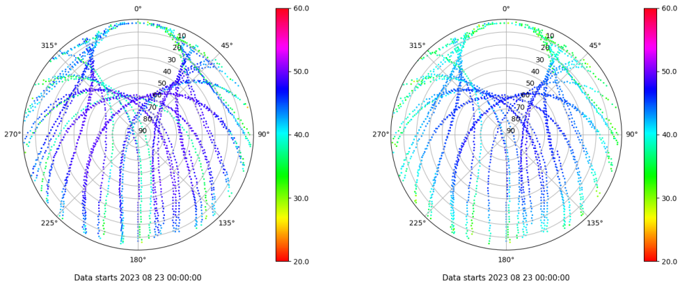
Skyplot for station JACA. Signal to Noise S1C Data file JACA00ESP_R_2023235.xtr Skyplot for station JACA. Signal to Noise S2P Data file JACA00ESP_R_2023235.xtr
