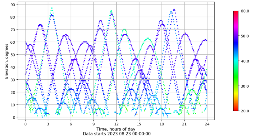
Time-elevation plot for station JACA. Signal to Noise S1C Data file JACA00ESP_R_2023235.xtr
