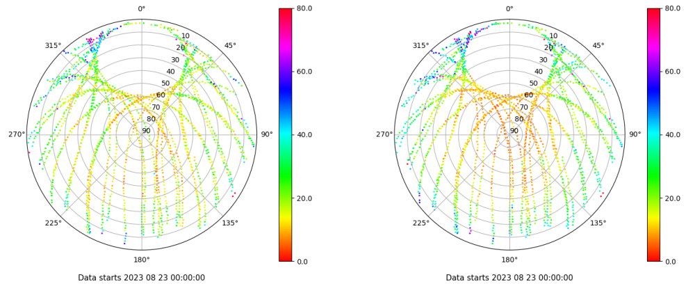
Skyplot for station JACA. Parameter M1C Data file JACA00ESP_R_2023235.xtr Skyplot for station JACA. Parameter M2P Data file JACA00ESP_R_2023235.xtr
