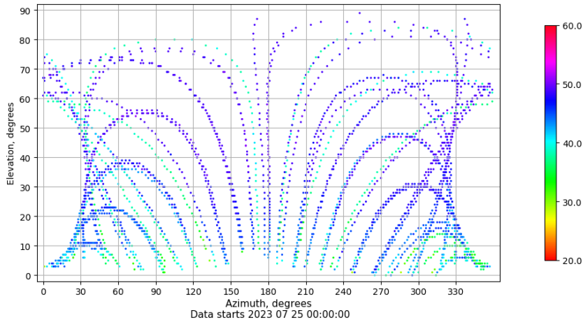
Azimuth-elevation plot for station JACA. Signal to Noise S1C Data file JACA00ESP_R_2023206.xtr
