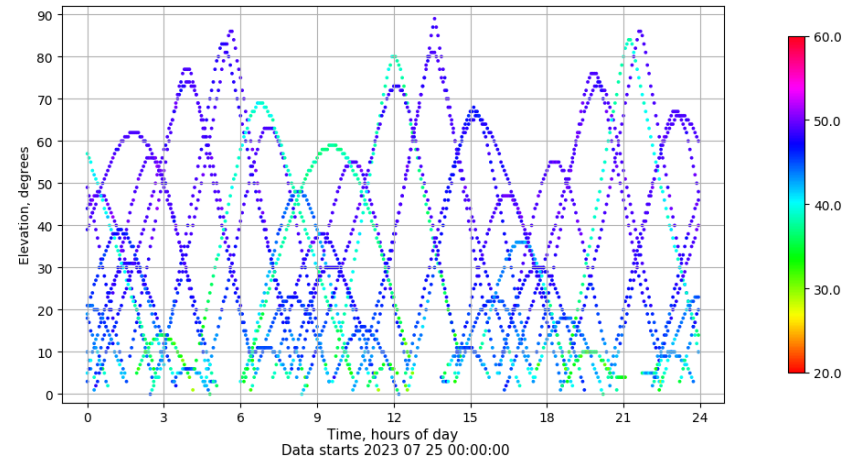
Time-elevation plot for station JACA. Signal to Noise S1C Data file JACA00ESP_R_2023206.xtr
