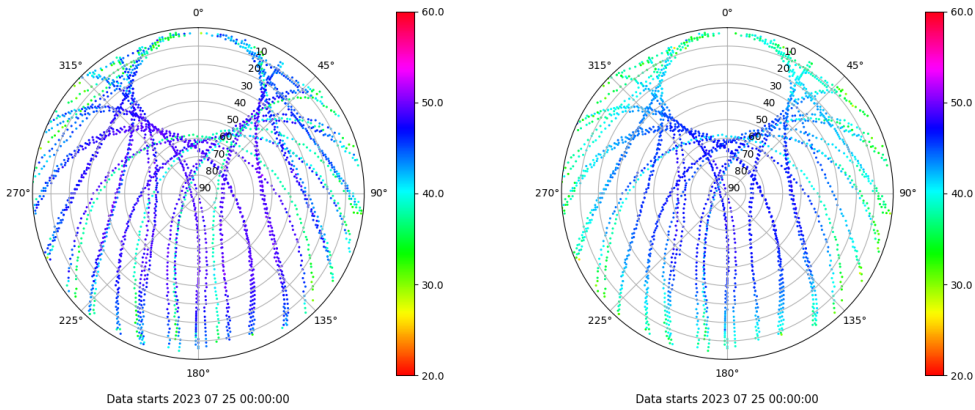
Skyplot for station JACA. Signal to Noise S1C Data file JACA00ESP_R_2023206.xtr Skyplot for station JACA. Signal to Noise S2P Data file JACA00ESP_R_2023206.xtr
