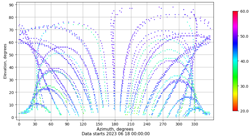
Azimuth-elevation plot for station JACA. Signal to Noise S1C Data file JACA00ESP_R_2023169.xtr
