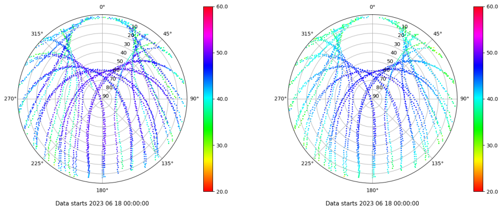
Skyplot for station JACA. Signal to Noise S1C Data file JACA00ESP_R_2023169.xtr Skyplot for station JACA. Signal to Noise S2P Data file JACA00ESP_R_2023169.xtr
