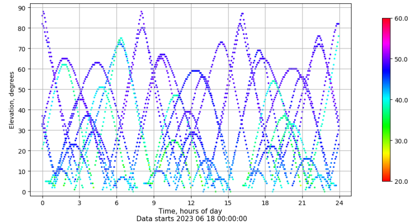
Time-elevation plot for station JACA. Signal to Noise S1C Data file JACA00ESP_R_2023169.xtr
