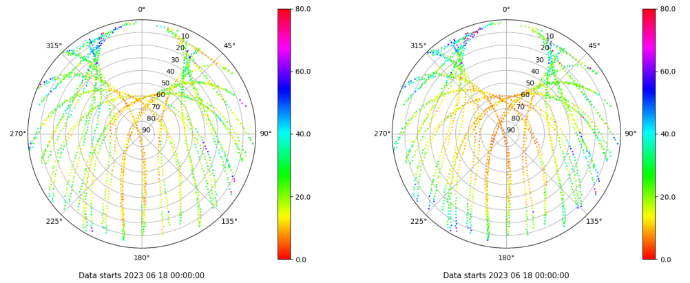
Skyplot for station JACA. Parameter M1C Data file JACA00ESP_R_2023169.xtr Skyplot for station JACA. Parameter M2P Data file JACA00ESP_R_2023169.xtr
