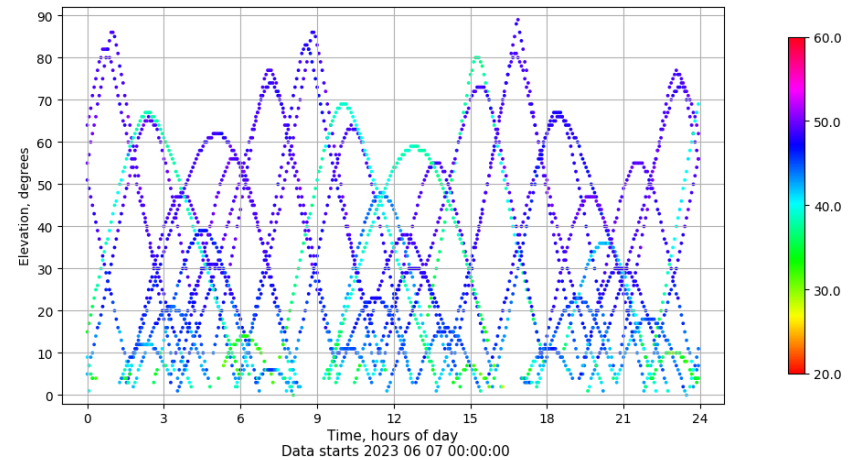
Time-elevation plot for station JACA. Signal to Noise S1C Data file JACA00ESP_R_2023158.xtr
