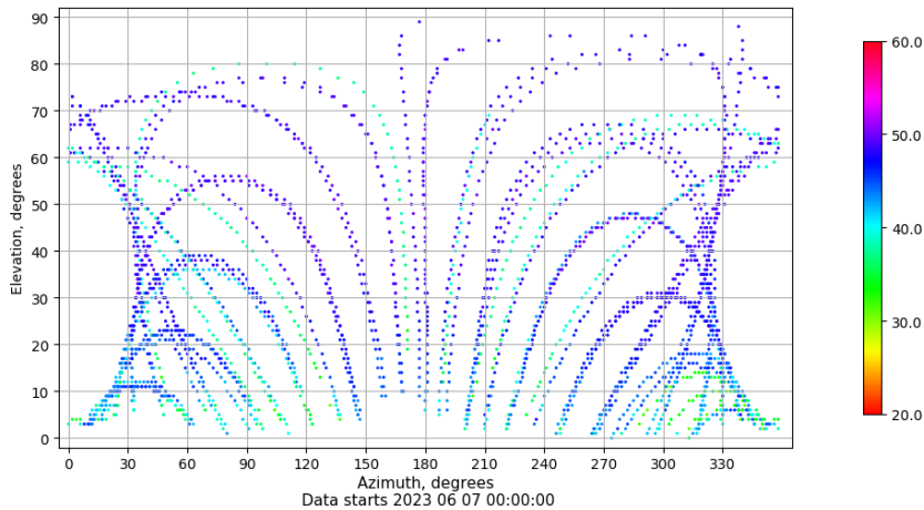
Azimuth-elevation plot for station JACA. Signal to Noise S1C Data file JACA00ESP_R_2023158.xtr
