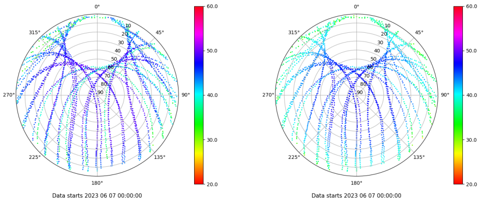
Skyplot for station JACA. Signal to Noise S1C Data file JACA00ESP_R_2023158.xtr Skyplot for station JACA. Signal to Noise S2P Data file JACA00ESP_R_2023158.xtr
