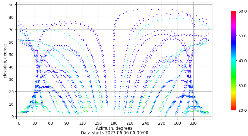
Azimuth-elevation plot for station JACA. Signal to Noise S1C Data file JACA00ESP_R_2023157.xtr
