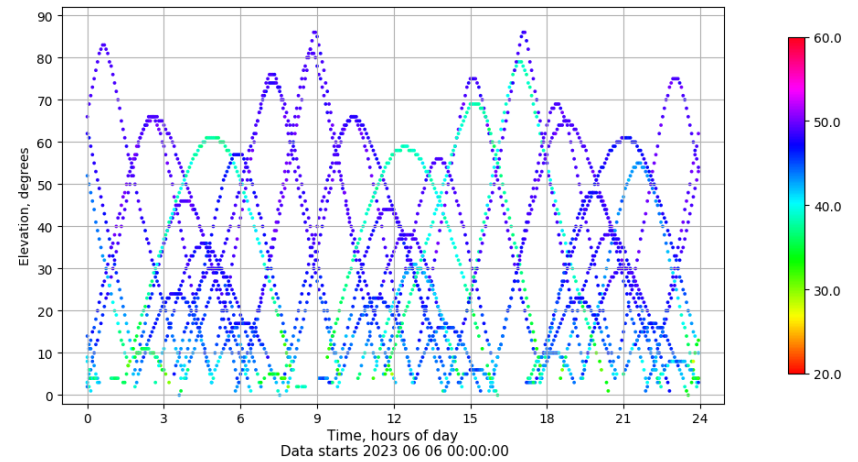
Time-elevation plot for station JACA. Signal to Noise S1C Data file JACA00ESP_R_2023157.xtr
