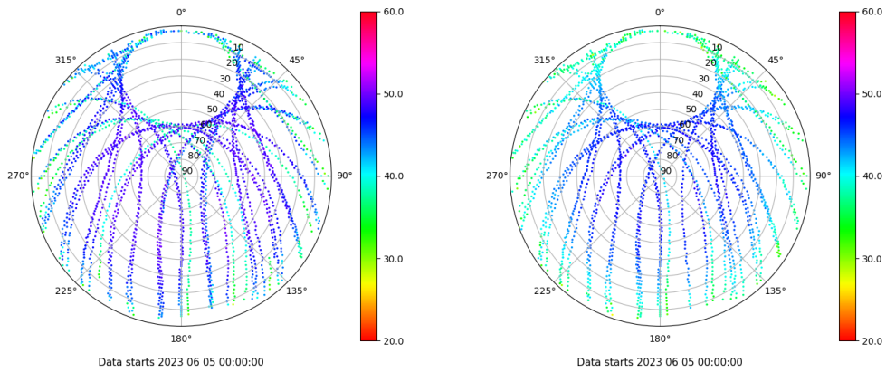
Skyplot for station JACA. Signal to Noise S1C Data file JACA00ESP_R_2023156.xtr Skyplot for station JACA. Signal to Noise S2P Data file JACA00ESP_R_2023156.xtr
