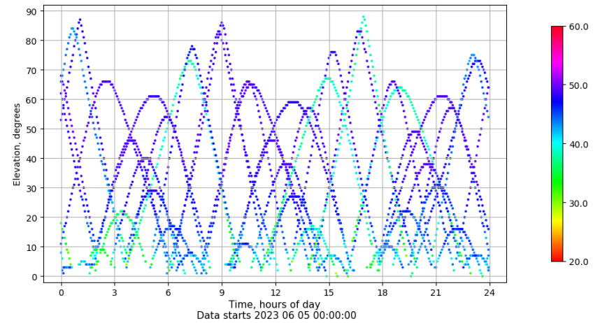
Time-elevation plot for station JACA. Signal to Noise S1C Data file JACA00ESP_R_2023156.xtr
