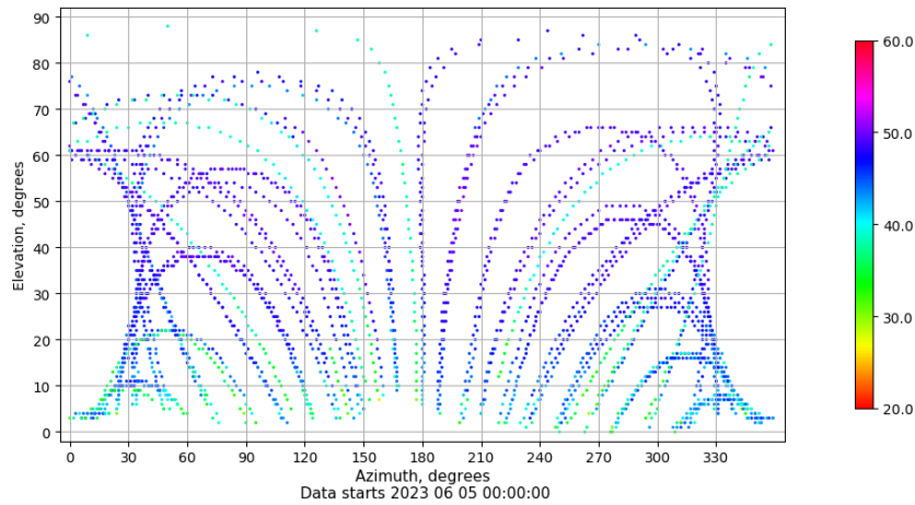
Azimuth-elevation plot for station JACA. Signal to Noise S1C Data file JACA00ESP_R_2023156.xtr
