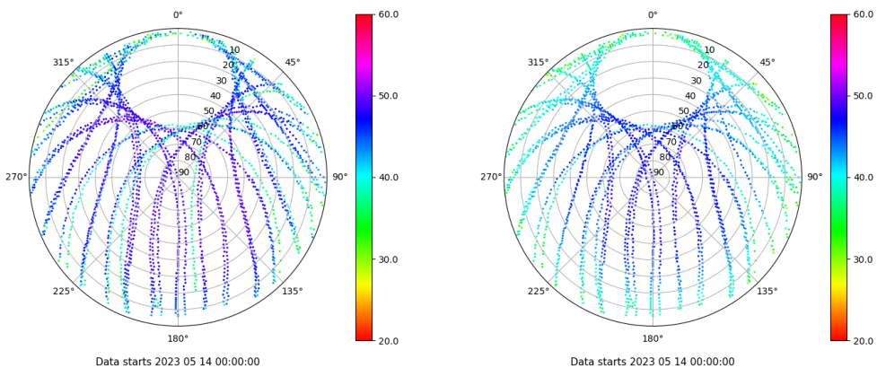
Skyplot for station JACA. Signal to Noise S1C Data file JACA00ESP_R_2023134.xtr Skyplot for station JACA. Signal to Noise S2P Data file JACA00ESP_R_2023134.xtr
