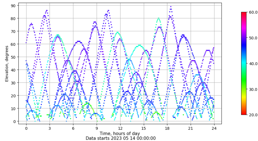
Time-elevation plot for station JACA. Signal to Noise S1C Data file JACA00ESP_R_2023134.xtr
