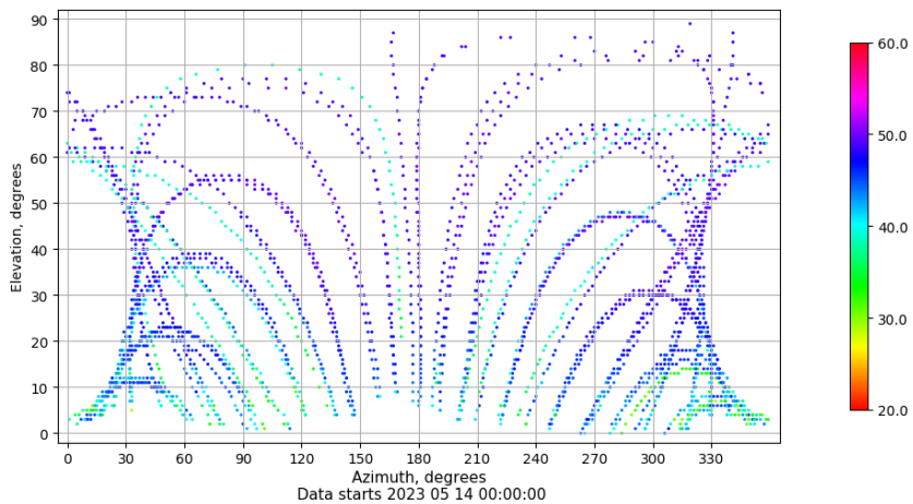
Azimuth-elevation plot for station JACA. Signal to Noise S1C Data file JACA00ESP_R_2023134.xtr
