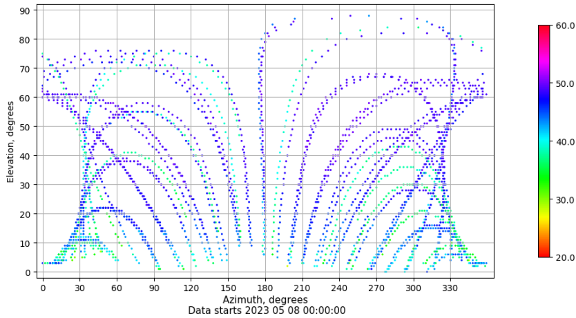
Azimuth-elevation plot for station JACA. Signal to Noise S1C Data file JACA00ESP_R_2023128.xtr
