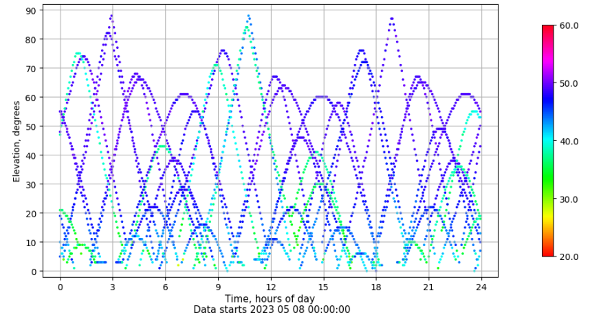
Time-elevation plot for station JACA. Signal to Noise S1C Data file JACA00ESP_R_2023128.xtr
