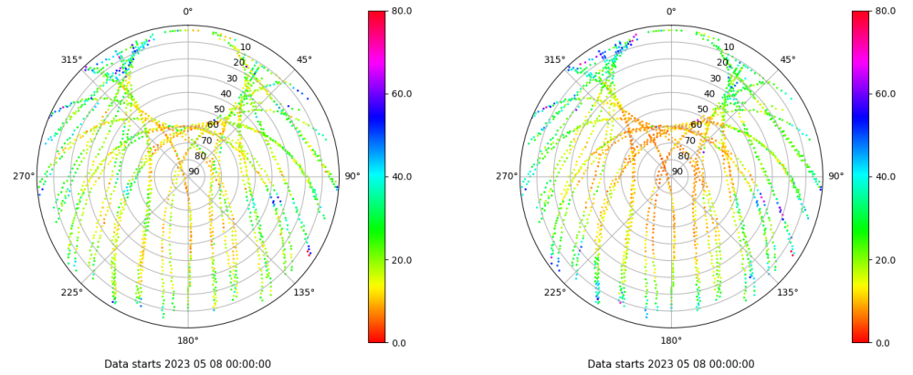
Skyplot for station JACA. Parameter M1C Data file JACA00ESP_R_2023128.xtr Skyplot for station JACA. Parameter M2P Data file JACA00ESP_R_2023128.xtr
