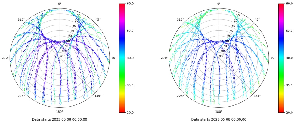
Skyplot for station JACA. Signal to Noise S1C Data file JACA00ESP_R_2023128.xtr Skyplot for station JACA. Signal to Noise S2P Data file JACA00ESP_R_2023128.xtr
