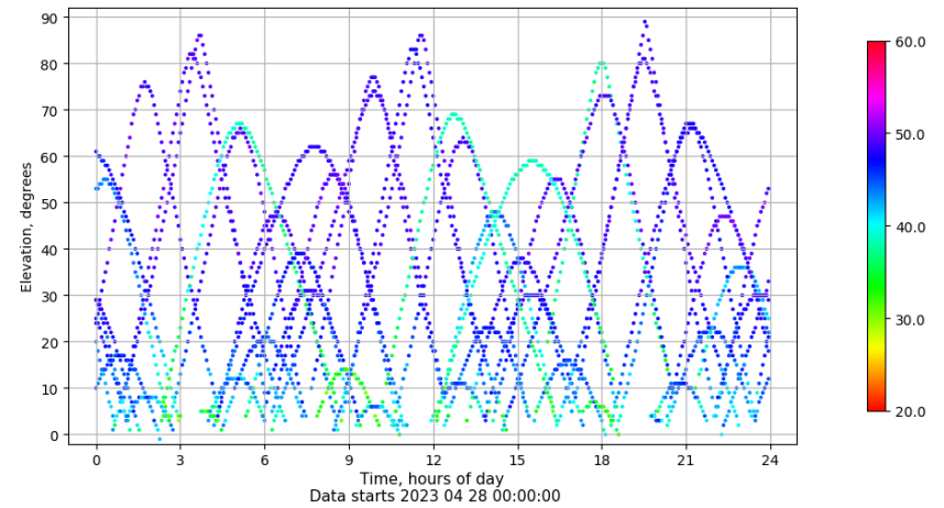
Time-elevation plot for station JACA. Signal to Noise S1C Data file JACA00ESP_R_2023118.xtr
