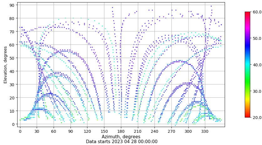
Azimuth-elevation plot for station JACA. Signal to Noise S1C Data file JACA00ESP_R_2023118.xtr
