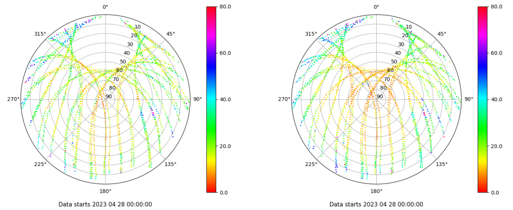
Skyplot for station JACA. Parameter M1C Data file JACA00ESP_R_2023118.xtr Skyplot for station JACA. Parameter M2P Data file JACA00ESP_R_2023118.xtr
