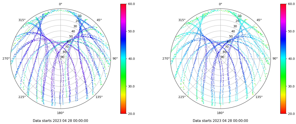
Skyplot for station JACA. Signal to Noise S1C Data file JACA00ESP_R_2023118.xtr Skyplot for station JACA. Signal to Noise S2P Data file JACA00ESP_R_2023118.xtr
