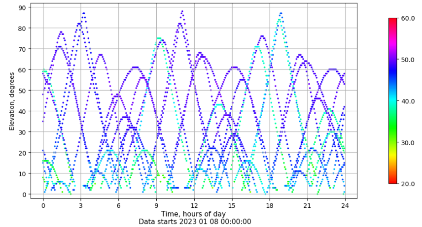
Time-elevation plot for station JACA. Signal to Noise S1C Data file JACA00ESP_R_2023008.xtr
