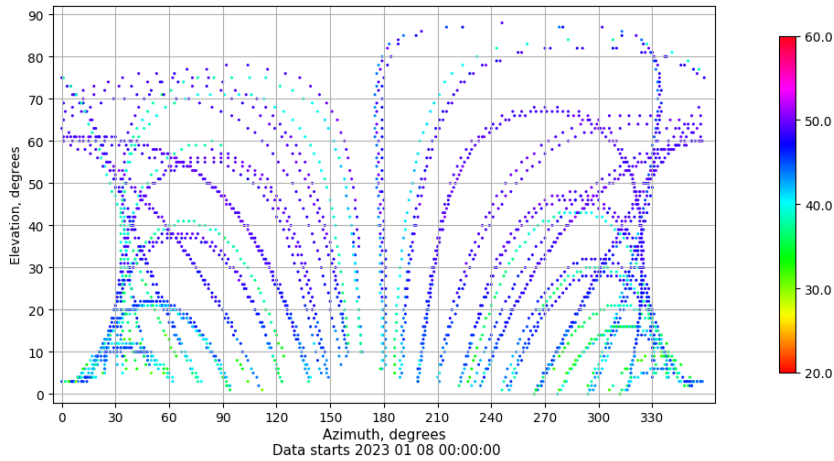
Azimuth-elevation plot for station JACA. Signal to Noise S1C Data file JACA00ESP_R_2023008.xtr
