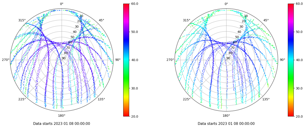
Skyplot for station JACA. Signal to Noise S1C Data file JACA00ESP_R_2023008.xtr Skyplot for station JACA. Signal to Noise S2P Data file JACA00ESP_R_2023008.xtr
