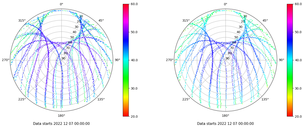
Skyplot for station JACA. Signal to Noise S1C Data file JACA00ESP_R_2022341.xtr Skyplot for station JACA. Signal to Noise S2P Data file JACA00ESP_R_2022341.xtr
