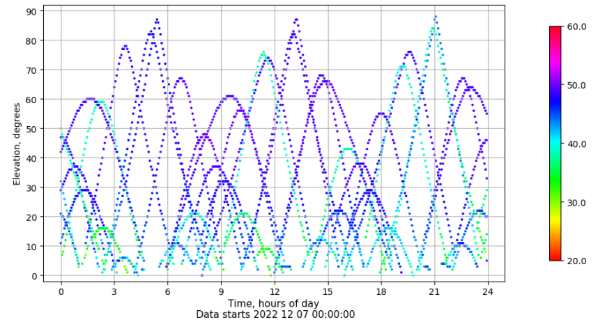
Time-elevation plot for station JACA. Signal to Noise S1C Data file JACA00ESP_R_2022341.xtr
