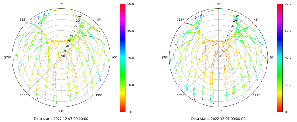
Skyplot for station JACA. Parameter M1C Data file JACA00ESP_R_2022341.xtr Skyplot for station JACA. Parameter M2P Data file JACA00ESP_R_2022341.xtr
