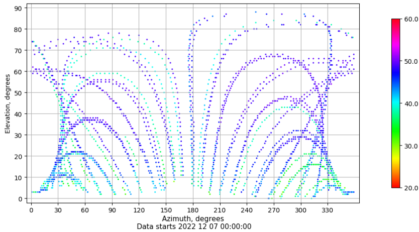
Azimuth-elevation plot for station JACA. Signal to Noise S1C Data file JACA00ESP_R_2022341.xtr
