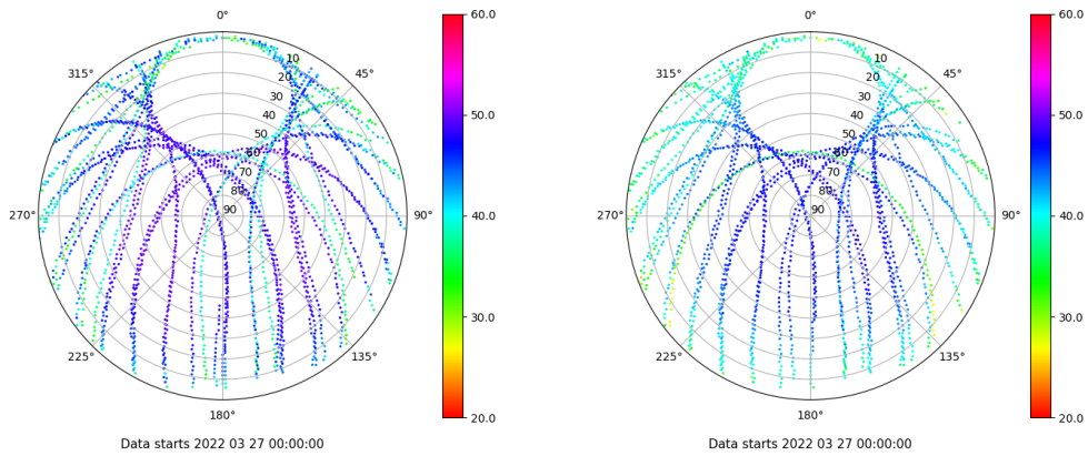
Skyplot for station JACA. Signal to Noise S1C Data file JACA00ESP_R_2022086.xtr Skyplot for station JACA. Signal to Noise S2P Data file JACA00ESP_R_2022086.xtr
