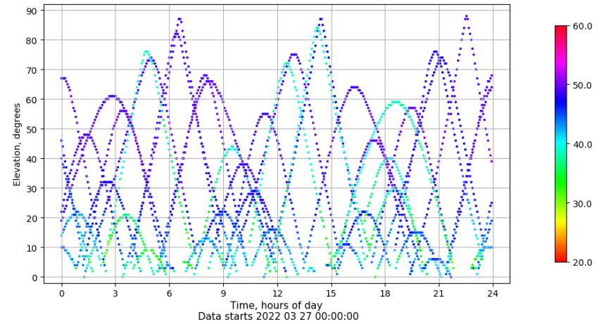
Time-elevation plot for station JACA. Signal to Noise S1C Data file JACA00ESP_R_2022086.xtr
