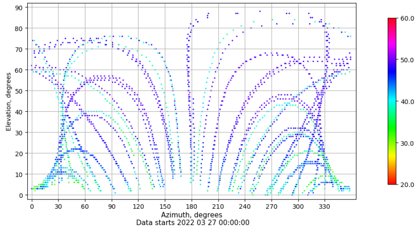
Azimuth-elevation plot for station JACA. Signal to Noise S1C Data file JACA00ESP_R_2022086.xtr
