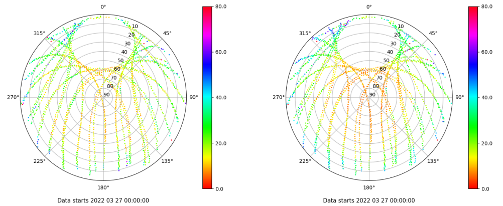
Skyplot for station JACA. Parameter M1C Data file JACA00ESP_R_2022086.xtr Skyplot for station JACA. Parameter M2P Data file JACA00ESP_R_2022086.xtr
