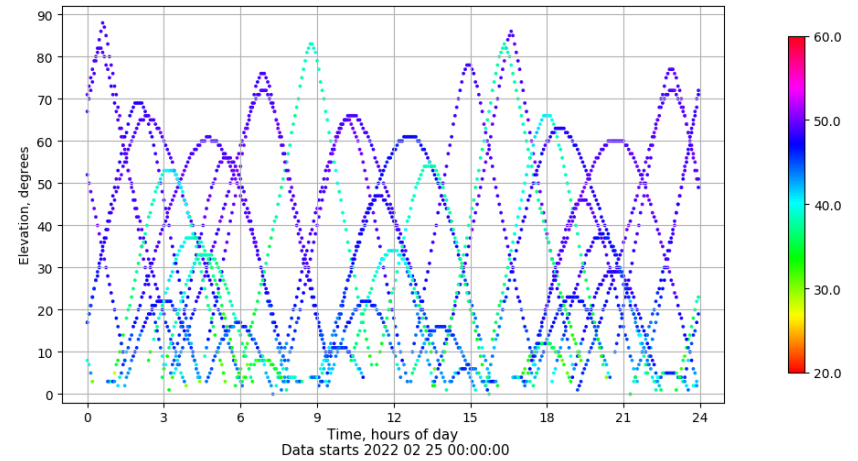
Time-elevation plot for station JACA. Signal to Noise S1C Data file JACA00ESP_R_2022056.xtr
