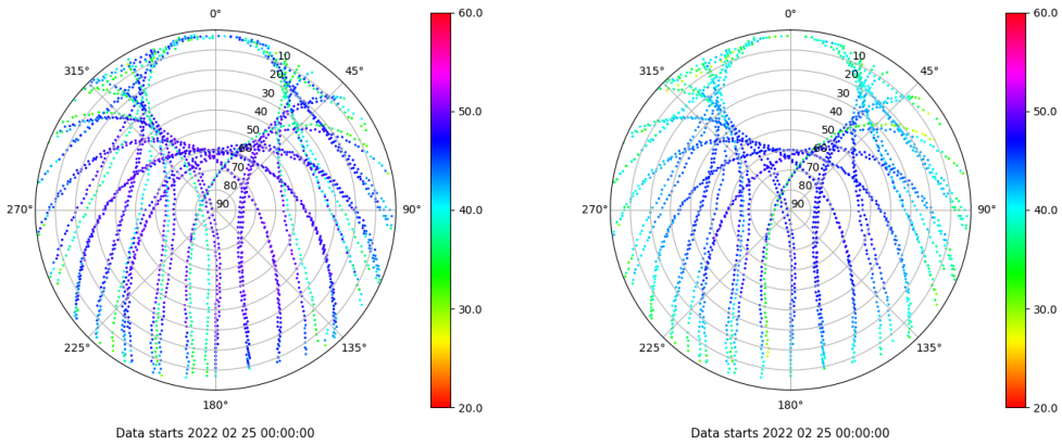
Skyplot for station JACA. Signal to Noise S1C Data file JACA00ESP_R_2022056.xtr Skyplot for station JACA. Signal to Noise S2P Data file JACA00ESP_R_2022056.xtr
