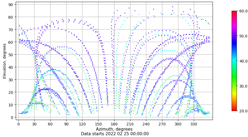
Azimuth-elevation plot for station JACA. Signal to Noise S1C Data file JACA00ESP_R_2022056.xtr
