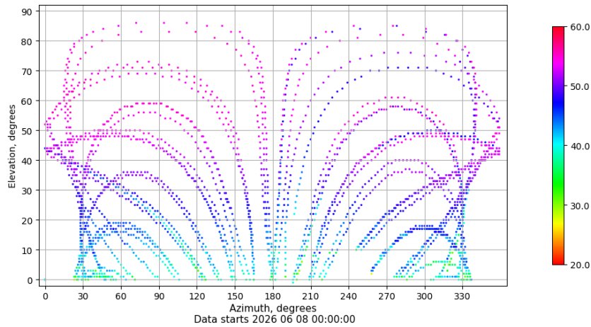
Azimuth-elevation plot for station IZAN. Signal to Noise S1C Data file IZAN00ESP_R_2026159.xtr
