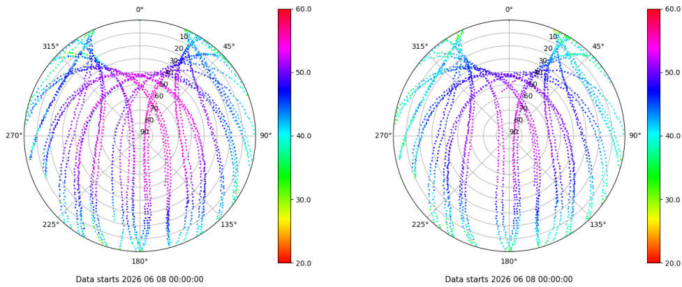
Skyplot for station IZAN. Signal to Noise S1C Data file IZAN00ESP_R_2026159.xtr Skyplot for station IZAN. Signal to Noise S2C Data file IZAN00ESP_R_2026159.xtr
