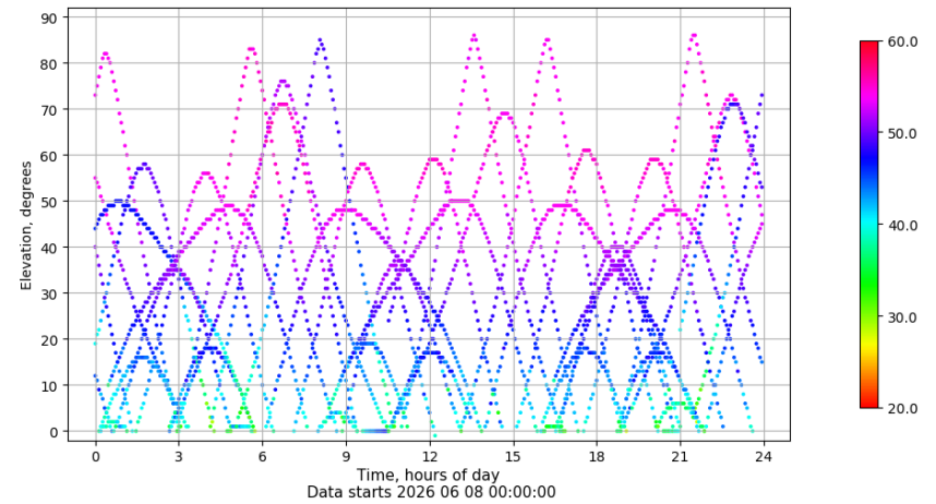
Time-elevation plot for station IZAN. Signal to Noise S1C Data file IZAN00ESP_R_2026159.xtr
