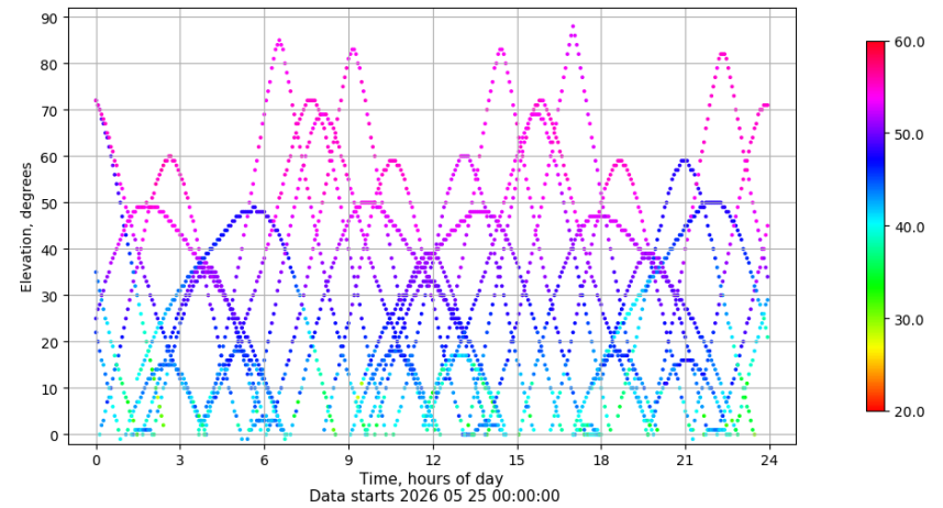
Time-elevation plot for station IZAN. Signal to Noise S1C Data file IZAN00ESP_R_2026145.xtr
