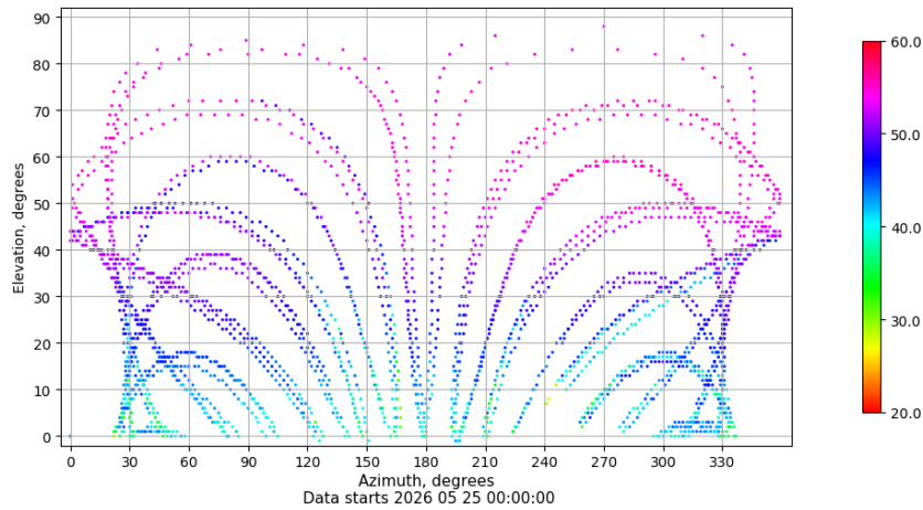
Azimuth-elevation plot for station IZAN. Signal to Noise S1C Data file IZAN00ESP_R_2026145.xtr
