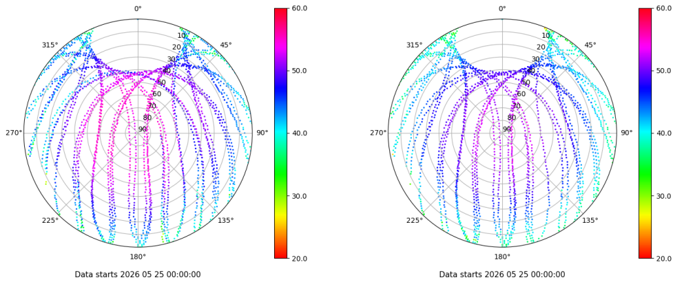
Skyplot for station IZAN. Signal to Noise S1C Data file IZAN00ESP_R_2026145.xtr Skyplot for station IZAN. Signal to Noise S2C Data file IZAN00ESP_R_2026145.xtr
