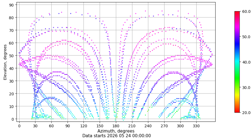
Azimuth-elevation plot for station IZAN. Signal to Noise S1C Data file IZAN00ESP_R_2026144.xtr
