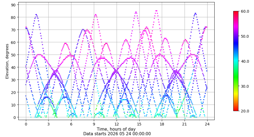
Time-elevation plot for station IZAN. Signal to Noise S1C Data file IZAN00ESP_R_2026144.xtr
