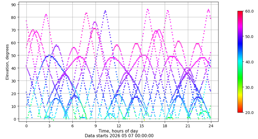
Time-elevation plot for station IZAN. Signal to Noise S1C Data file IZAN00ESP_R_2026127.xtr
