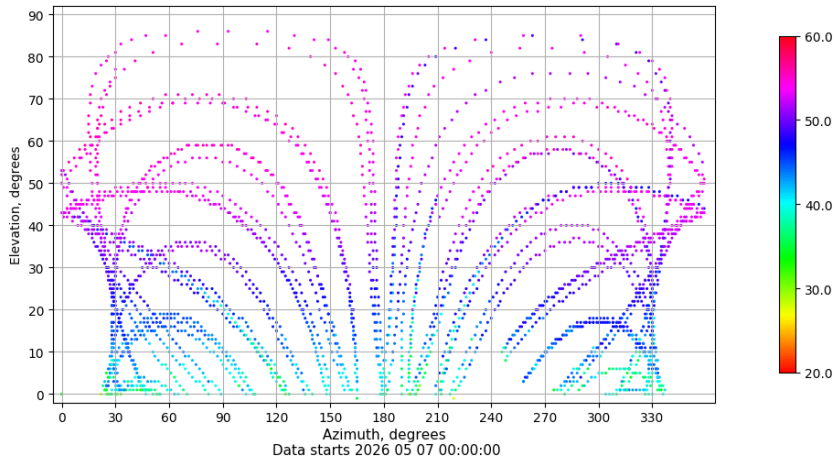
Azimuth-elevation plot for station IZAN. Signal to Noise S1C Data file IZAN00ESP_R_2026127.xtr
