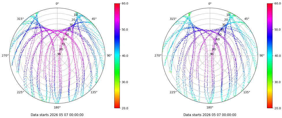
Skyplot for station IZAN. Signal to Noise S1C Data file IZAN00ESP_R_2026127.xtr Skyplot for station IZAN. Signal to Noise S2C Data file IZAN00ESP_R_2026127.xtr
