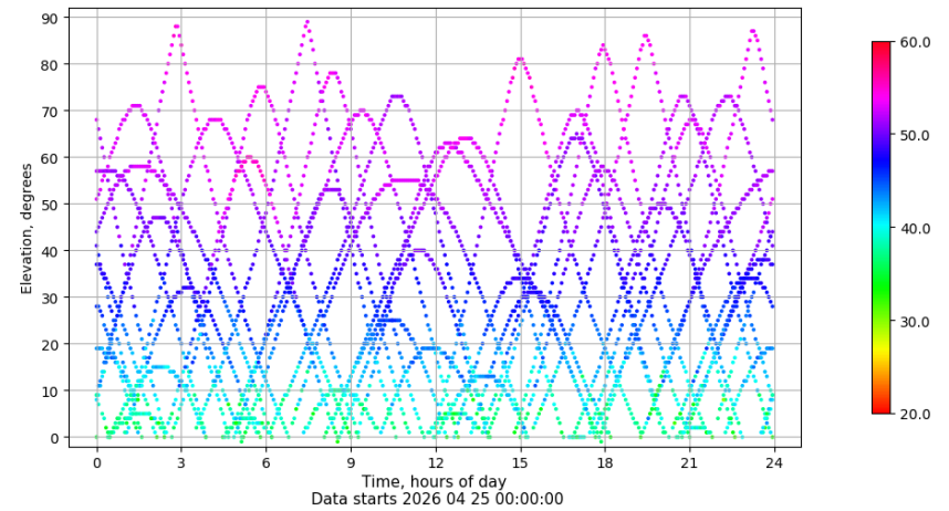
Time-elevation plot for station IZAN. Signal to Noise S1C Data file IZAN00ESP_R_2026115.xtr
