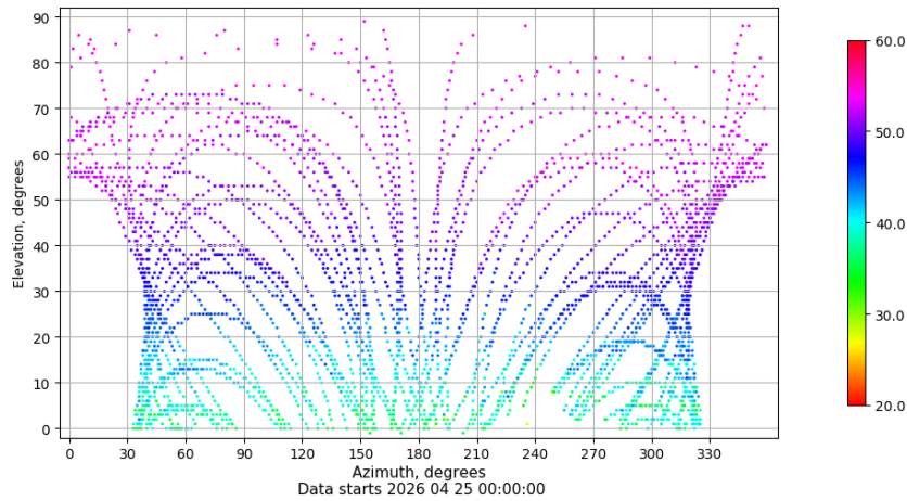
Azimuth-elevation plot for station IZAN. Signal to Noise S1C Data file IZAN00ESP_R_2026115.xtr
