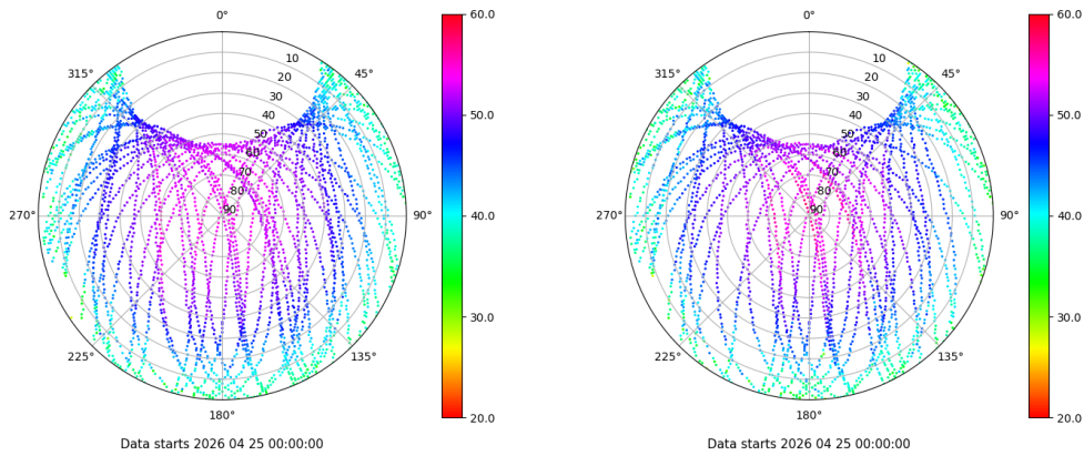
Skyplot for station IZAN. Signal to Noise S1C Data file IZAN00ESP_R_2026115.xtr Skyplot for station IZAN. Signal to Noise S2S Data file IZAN00ESP_R_2026115.xtr
