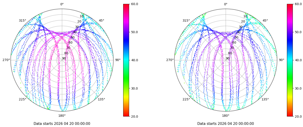
Skyplot for station IZAN. Signal to Noise S1C Data file IZAN00ESP_R_2026110.xtr Skyplot for station IZAN. Signal to Noise S2C Data file IZAN00ESP_R_2026110.xtr
