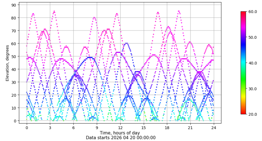
Time-elevation plot for station IZAN. Signal to Noise S1C Data file IZAN00ESP_R_2026110.xtr
