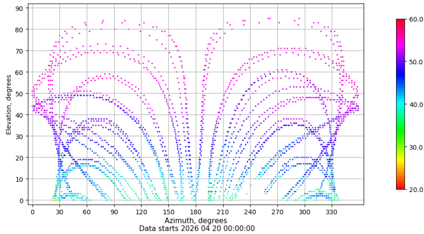
Azimuth-elevation plot for station IZAN. Signal to Noise S1C Data file IZAN00ESP_R_2026110.xtr
