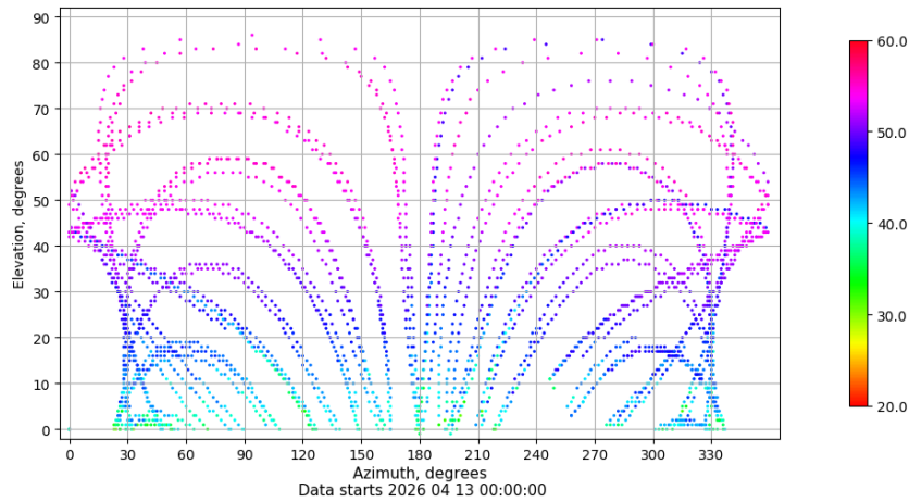
Azimuth-elevation plot for station IZAN. Signal to Noise S1C Data file IZAN00ESP_R_2026103.xtr
