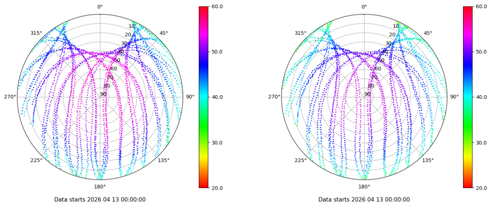
Skyplot for station IZAN. Signal to Noise S1C Data file IZAN00ESP_R_2026103.xtr Skyplot for station IZAN. Signal to Noise S2C Data file IZAN00ESP_R_2026103.xtr
