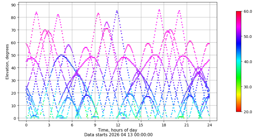
Time-elevation plot for station IZAN. Signal to Noise S1C Data file IZAN00ESP_R_2026103.xtr
