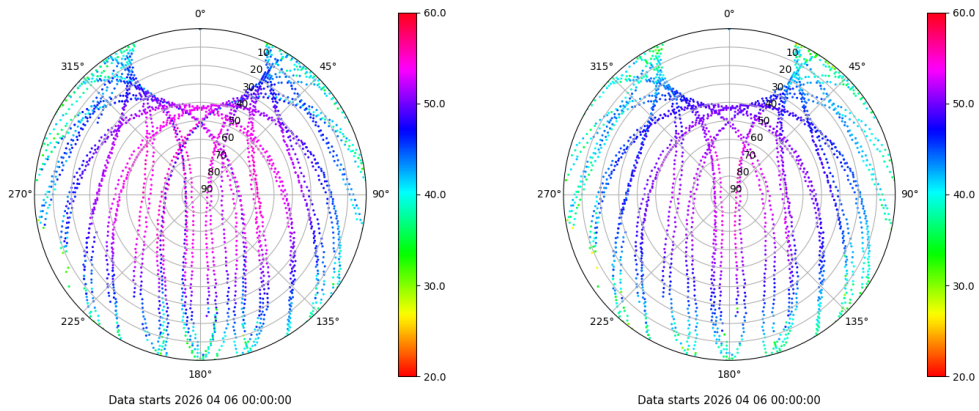
Skyplot for station IZAN. Signal to Noise S1C Data file IZAN00ESP_R_2026096.xtr Skyplot for station IZAN. Signal to Noise S2C Data file IZAN00ESP_R_2026096.xtr
