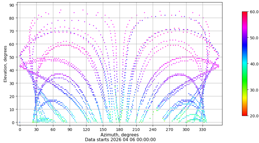
Azimuth-elevation plot for station IZAN. Signal to Noise S1C Data file IZAN00ESP_R_2026096.xtr
