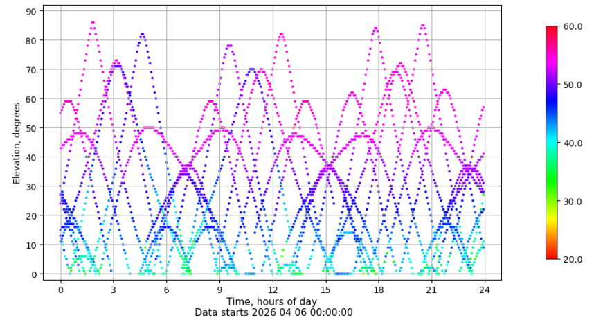
Time-elevation plot for station IZAN. Signal to Noise S1C Data file IZAN00ESP_R_2026096.xtr
