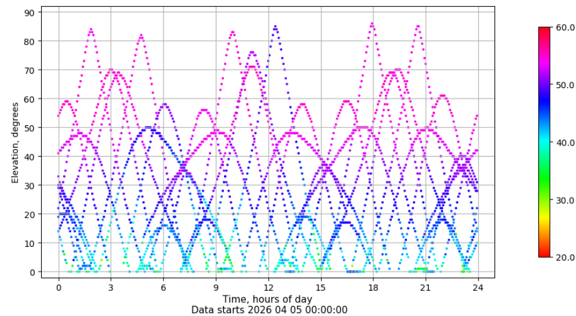
Time-elevation plot for station IZAN. Signal to Noise S1C Data file IZAN00ESP_R_2026095.xtr
