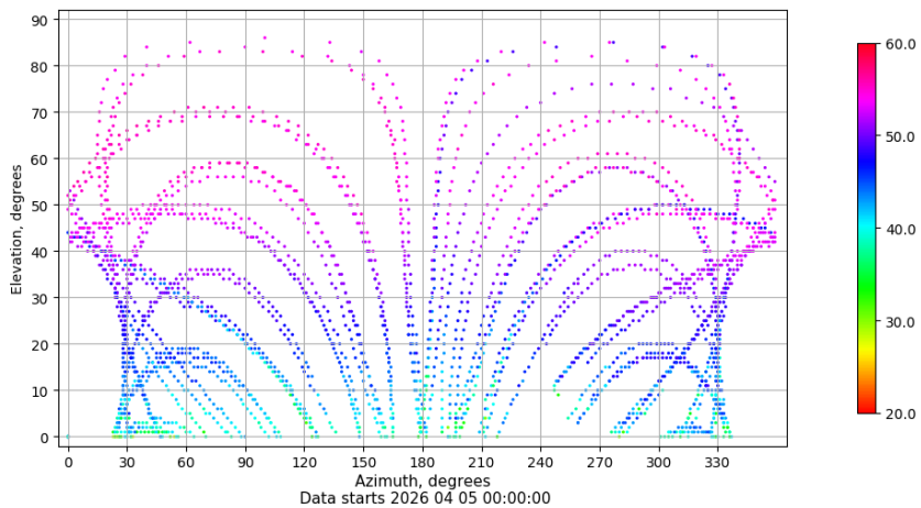
Azimuth-elevation plot for station IZAN. Signal to Noise S1C Data file IZAN00ESP_R_2026095.xtr
