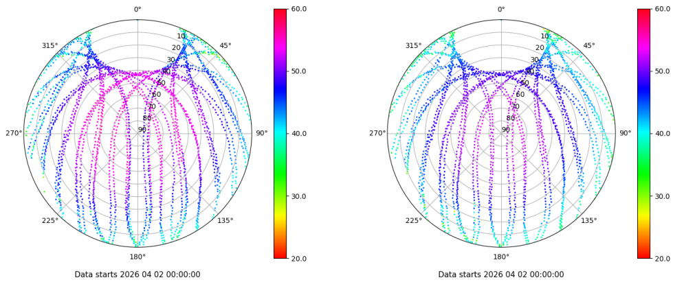
Skyplot for station IZAN. Signal to Noise S1C Data file IZAN00ESP_R_2026092.xtr Skyplot for station IZAN. Signal to Noise S2C Data file IZAN00ESP_R_2026092.xtr
