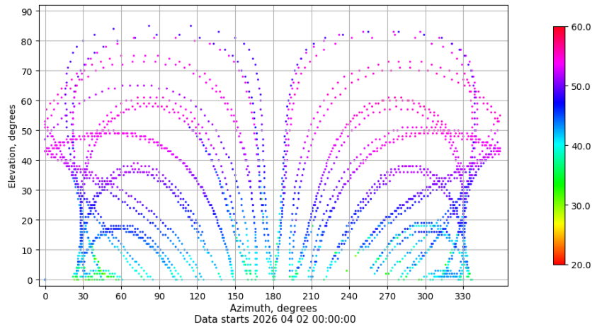
Azimuth-elevation plot for station IZAN. Signal to Noise S1C Data file IZAN00ESP_R_2026092.xtr
