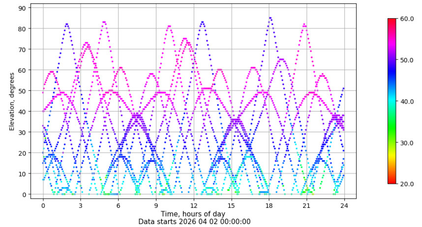
Time-elevation plot for station IZAN. Signal to Noise S1C Data file IZAN00ESP_R_2026092.xtr
