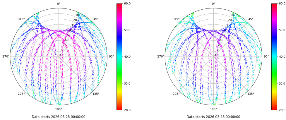
Skyplot for station IZAN. Signal to Noise S1C Data file IZAN00ESP_R_2026087.xtr Skyplot for station IZAN. Signal to Noise S2C Data file IZAN00ESP_R_2026087.xtr
