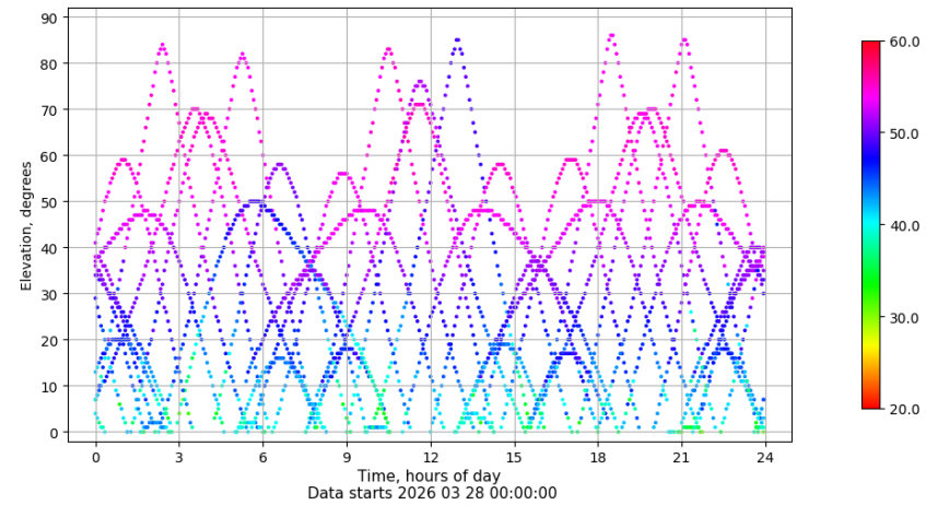
Time-elevation plot for station IZAN. Signal to Noise S1C Data file IZAN00ESP_R_2026087.xtr
