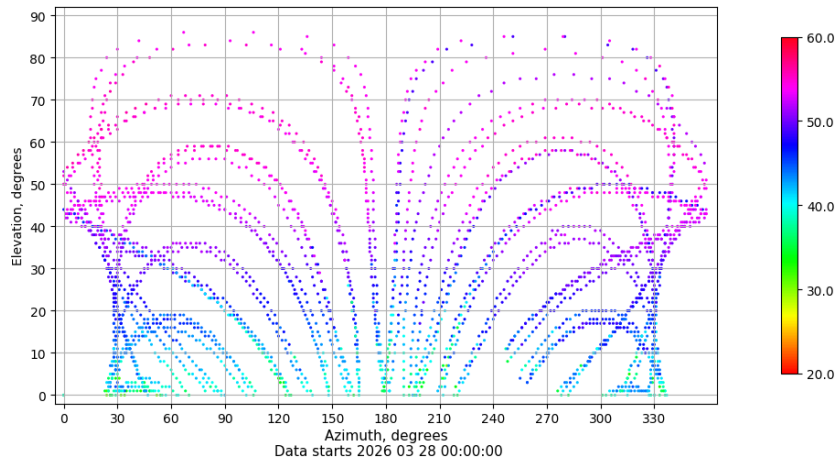
Azimuth-elevation plot for station IZAN. Signal to Noise S1C Data file IZAN00ESP_R_2026087.xtr
