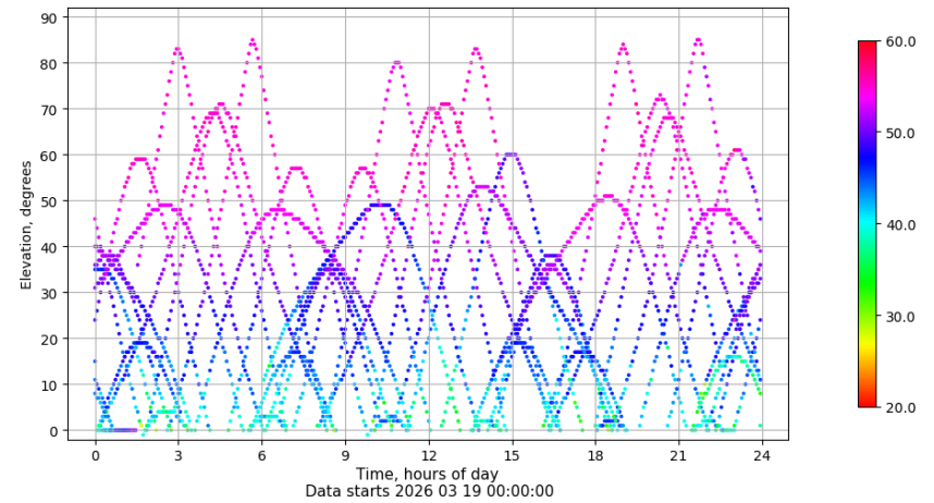
Time-elevation plot for station IZAN. Signal to Noise S1C Data file IZAN00ESP_R_2026078.xtr
