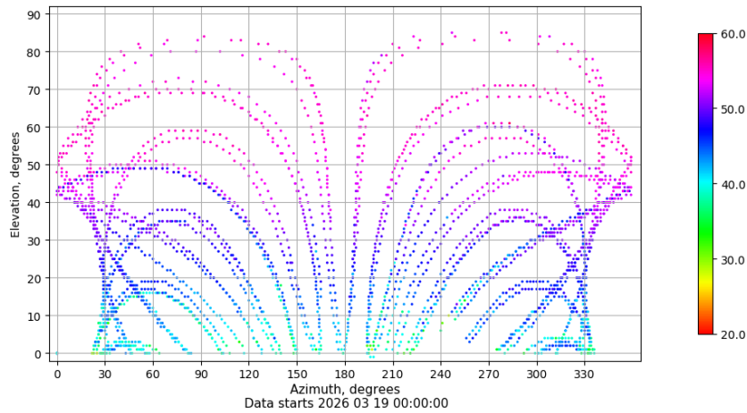
Azimuth-elevation plot for station IZAN. Signal to Noise S1C Data file IZAN00ESP_R_2026078.xtr
