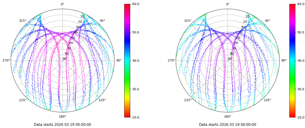
Skyplot for station IZAN. Signal to Noise S1C Data file IZAN00ESP_R_2026078.xtr Skyplot for station IZAN. Signal to Noise S2C Data file IZAN00ESP_R_2026078.xtr
