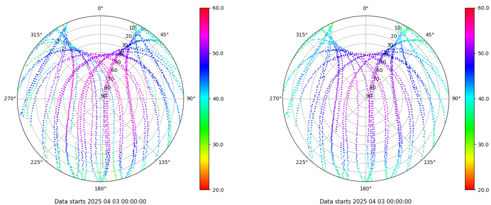
Skyplot for station IZAN. Signal to Noise S1C Data file IZAN00ESP_R_2025093.xtr Skyplot for station IZAN. Signal to Noise S2C Data file IZAN00ESP_R_2025093.xtr
