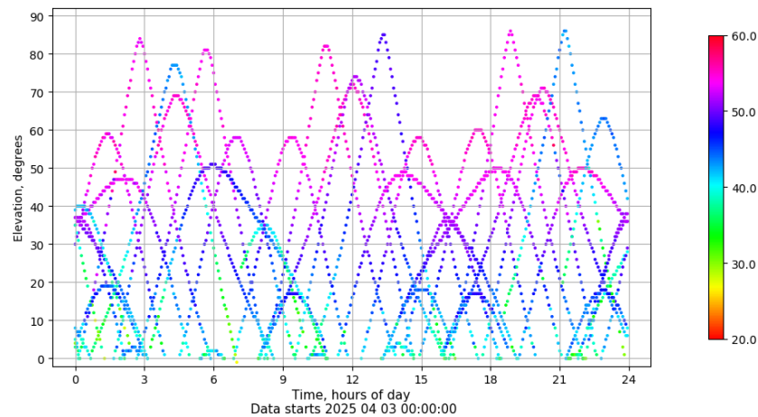
Time-elevation plot for station IZAN. Signal to Noise S1C Data file IZAN00ESP_R_2025093.xtr
