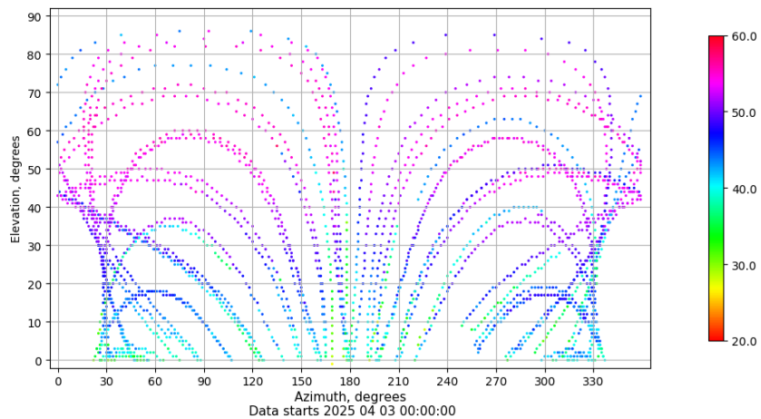
Azimuth-elevation plot for station IZAN. Signal to Noise S1C Data file IZAN00ESP_R_2025093.xtr
