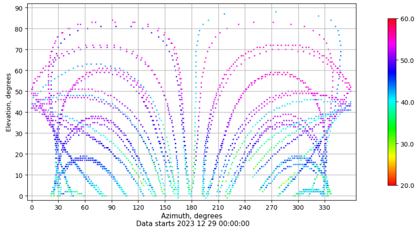
Azimuth-elevation plot for station IZAN. Signal to Noise S1C Data file IZAN00ESP_R_2023363.xtr
