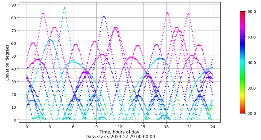
Time-elevation plot for station IZAN. Signal to Noise S1C Data file IZAN00ESP_R_2023363.xtr
