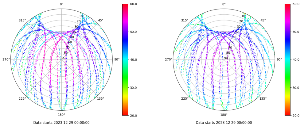
Skyplot for station IZAN. Signal to Noise S1C Data file IZAN00ESP_R_2023363.xtr Skyplot for station IZAN. Signal to Noise S2C Data file IZAN00ESP_R_2023363.xtr
