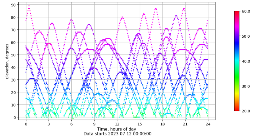
Time-elevation plot for station IZAN. Signal to Noise S1C Data file IZAN00ESP_R_2023193.xtr
