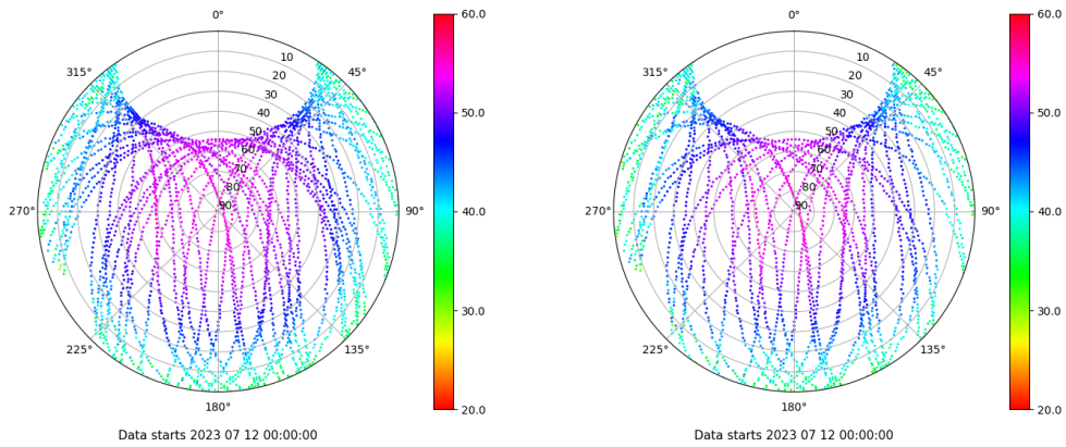
Skyplot for station IZAN. Signal to Noise S1C Data file IZAN00ESP_R_2023193.xtr Skyplot for station IZAN. Signal to Noise S2S Data file IZAN00ESP_R_2023193.xtr
