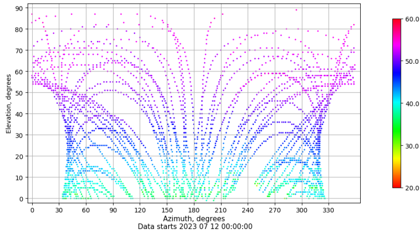
Azimuth-elevation plot for station IZAN. Signal to Noise S1C Data file IZAN00ESP_R_2023193.xtr
