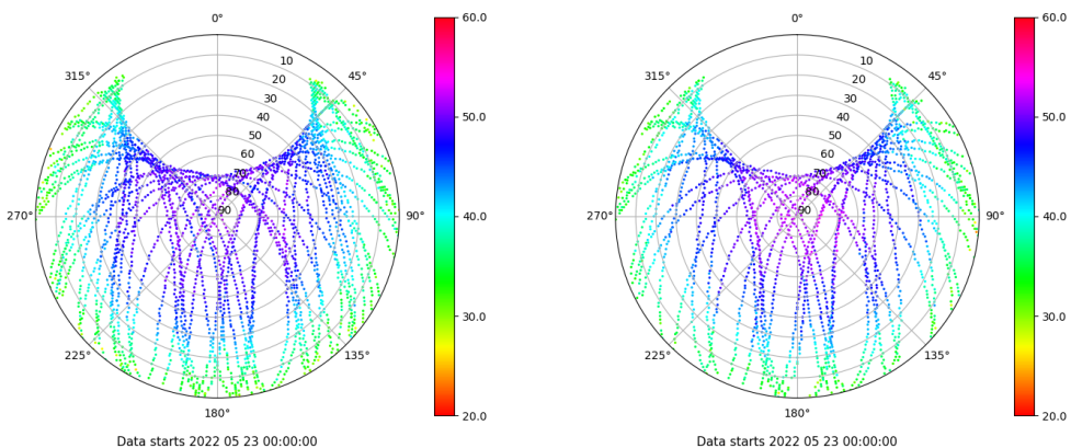
Skyplot for station ICOL. Signal to Noise S1C Data file ICOL00ESP_R_2022143.xtr Skyplot for station ICOL. Signal to Noise S2X Data file ICOL00ESP_R_2022143.xtr
