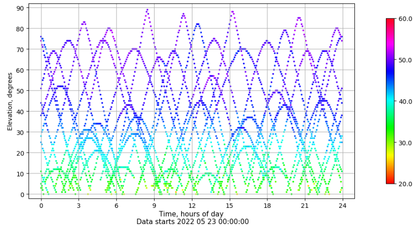
Time-elevation plot for station ICOL. Signal to Noise S1C Data file ICOL00ESP_R_2022143.xtr
