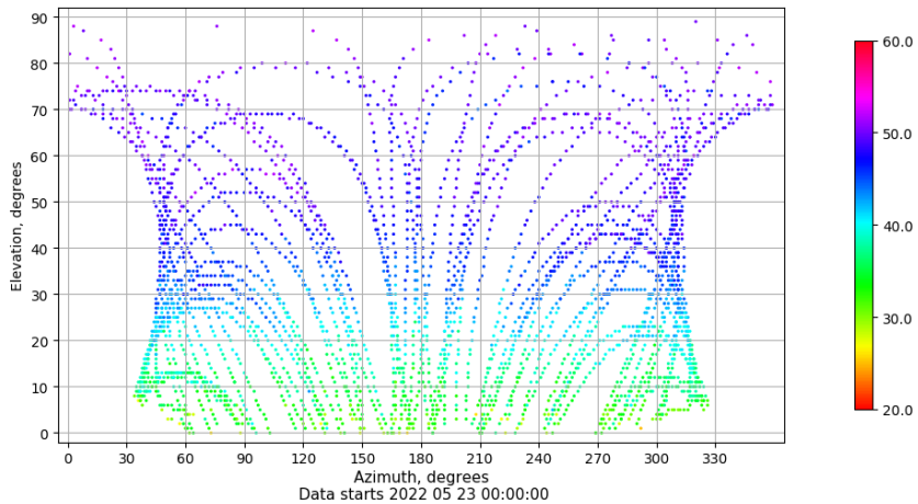
Azimuth-elevation plot for station ICOL. Signal to Noise S1C Data file ICOL00ESP_R_2022143.xtr
