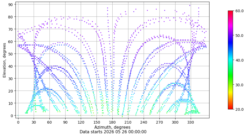
Azimuth-elevation plot for station IBIZ. Signal to Noise S1C Data file IBIZ00ESP_R_2026146.xtr
