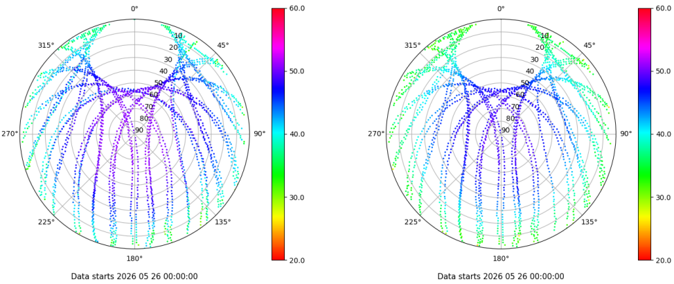
Skyplot for station IBIZ. Signal to Noise S1C Data file IBIZ00ESP_R_2026146.xtr Skyplot for station IBIZ. Signal to Noise S2P Data file IBIZ00ESP_R_2026146.xtr
