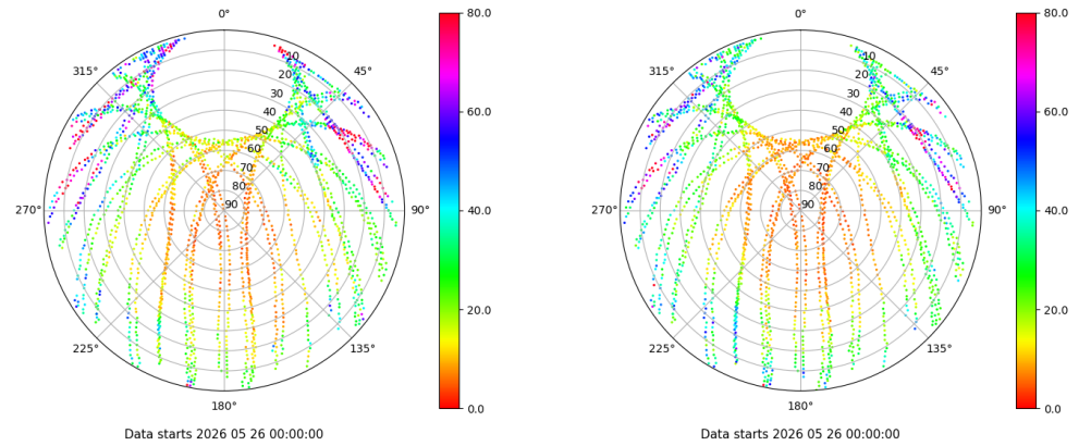
Skyplot for station IBIZ. Parameter M1C Data file IBIZ00ESP_R_2026146.xtr Skyplot for station IBIZ. Parameter M2P Data file IBIZ00ESP_R_2026146.xtr
