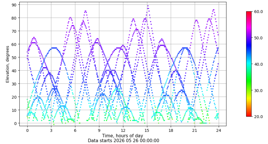
Time-elevation plot for station IBIZ. Signal to Noise S1C Data file IBIZ00ESP_R_2026146.xtr
