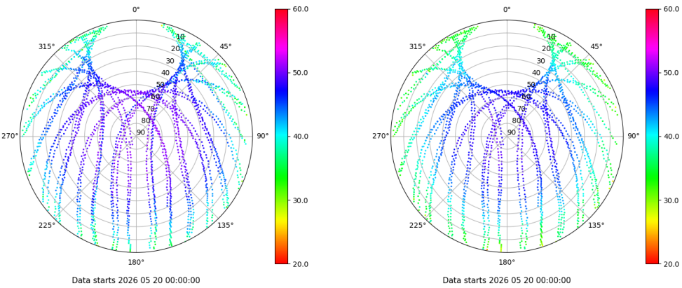
Skyplot for station IBIZ. Signal to Noise S1C Data file IBIZ00ESP_R_2026140.xtr Skyplot for station IBIZ. Signal to Noise S2P Data file IBIZ00ESP_R_2026140.xtr
