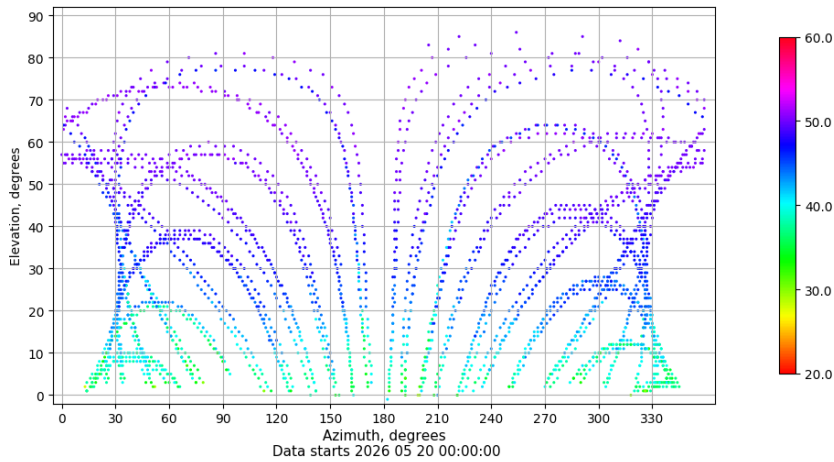
Azimuth-elevation plot for station IBIZ. Signal to Noise S1C Data file IBIZ00ESP_R_2026140.xtr
