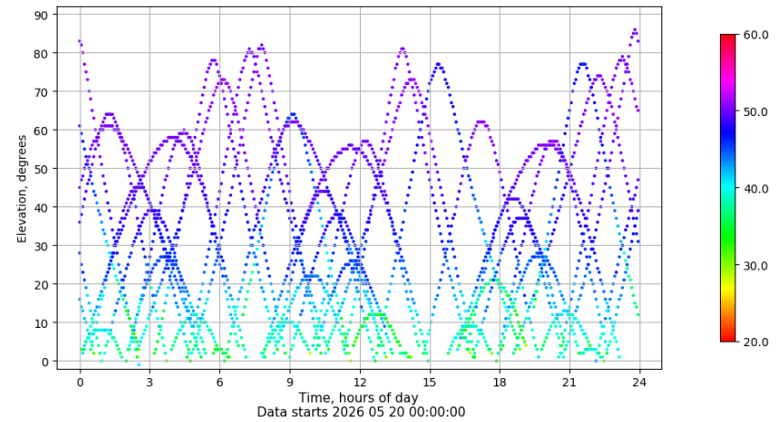
Time-elevation plot for station IBIZ. Signal to Noise S1C Data file IBIZ00ESP_R_2026140.xtr
