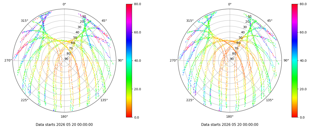
Skyplot for station IBIZ. Parameter M1C Data file IBIZ00ESP_R_2026140.xtr Skyplot for station IBIZ. Parameter M2P Data file IBIZ00ESP_R_2026140.xtr
