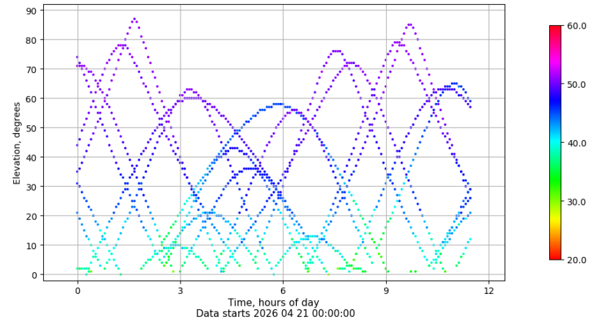
Time-elevation plot for station IBIZ. Signal to Noise S1C Data file IBIZ00ESP_R_2026111.xtr
