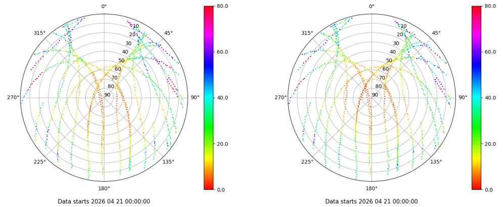
Skyplot for station IBIZ. Parameter M1C Data file IBIZ00ESP_R_2026111.xtr Skyplot for station IBIZ. Parameter M2P Data file IBIZ00ESP_R_2026111.xtr
