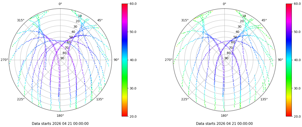
Skyplot for station IBIZ. Signal to Noise S1C Data file IBIZ00ESP_R_2026111.xtr Skyplot for station IBIZ. Signal to Noise S2P Data file IBIZ00ESP_R_2026111.xtr
