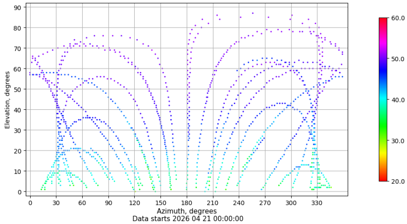
Azimuth-elevation plot for station IBIZ. Signal to Noise S1C Data file IBIZ00ESP_R_2026111.xtr
