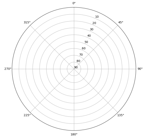
Skyplot for station IBIZ. Parameter M2W Data file IBIZ00ESP_R_2024110.xtr
