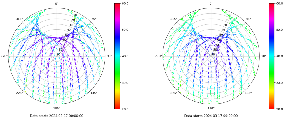
Skyplot for station IBIZ. Signal to Noise S1C Data file IBIZ00ESP_R_2024077.xtr Skyplot for station IBIZ. Signal to Noise S2P Data file IBIZ00ESP_R_2024077.xtr
