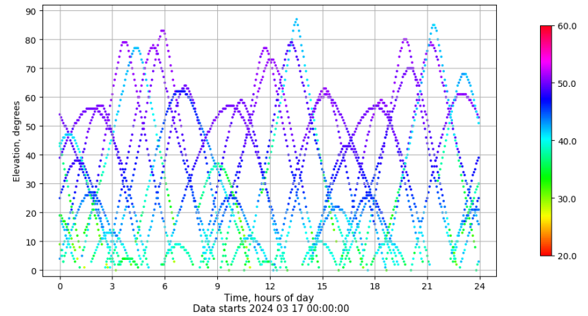
Time-elevation plot for station IBIZ. Signal to Noise S1C Data file IBIZ00ESP_R_2024077.xtr
