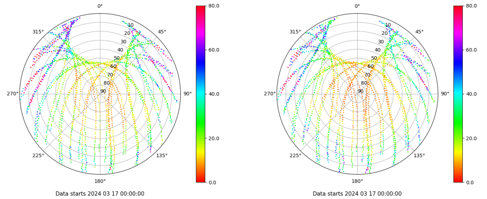
Skyplot for station IBIZ. Parameter M1C Data file IBIZ00ESP_R_2024077.xtr Skyplot for station IBIZ. Parameter M2P Data file IBIZ00ESP_R_2024077.xtr
