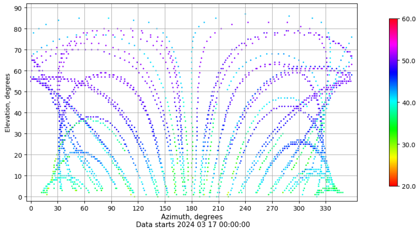
Azimuth-elevation plot for station IBIZ. Signal to Noise S1C Data file IBIZ00ESP_R_2024077.xtr
