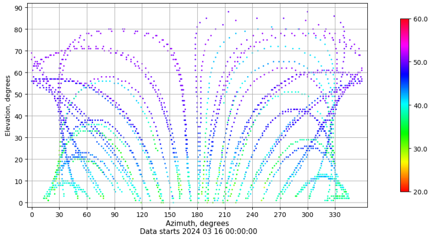
Azimuth-elevation plot for station IBIZ. Signal to Noise S1C Data file IBIZ00ESP_R_2024076.xtr
