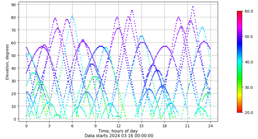
Time-elevation plot for station IBIZ. Signal to Noise S1C Data file IBIZ00ESP_R_2024076.xtr
