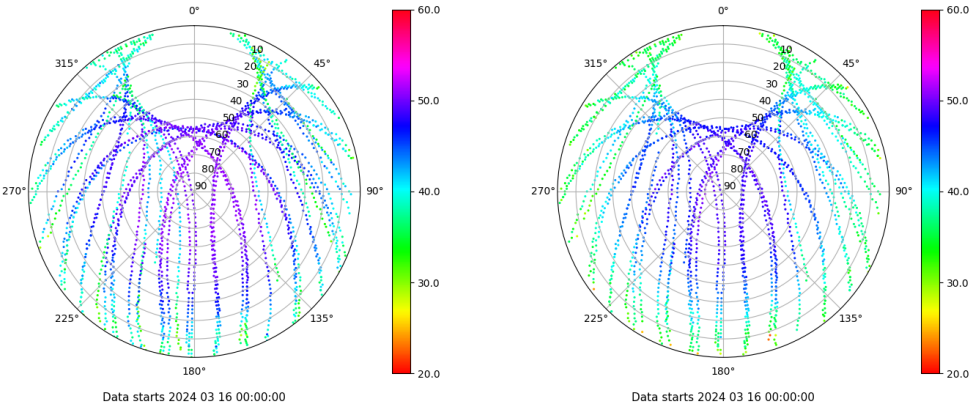
Skyplot for station IBIZ. Signal to Noise S1C Data file IBIZ00ESP_R_2024076.xtr Skyplot for station IBIZ. Signal to Noise S2P Data file IBIZ00ESP_R_2024076.xtr
